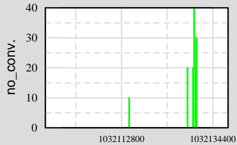
Ch 1: H0:PEM-LVEA_DST1_5
