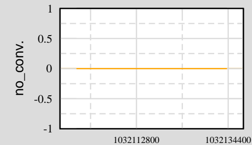
Ch 9: H0:PEM-LVEA_DST16_5
