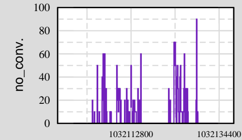
Ch 9: H0:PEM-LVEA_DST16_5
