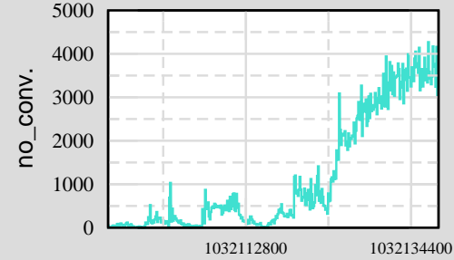
Ch 11: H0:PEM-EY_DST1_5
