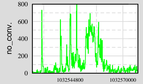
Ch 14: H0:PEM-LAB_DST2_3
