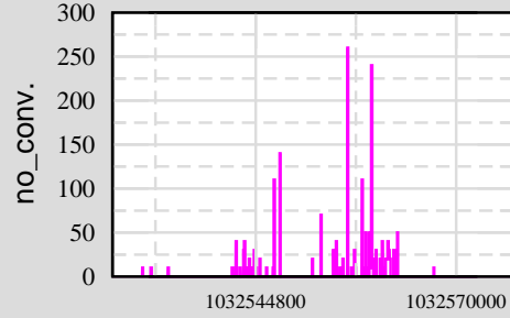
Ch 7: H0:PEM-LVEA_DST14_3
