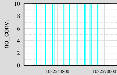
Ch 6: H0:PEM-LVEA_DST10_3
