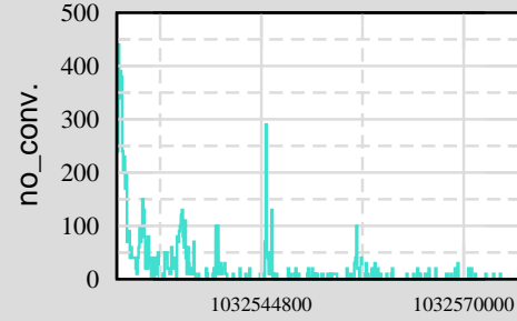
Ch 11: H0:PEM-EY_DST1_3
