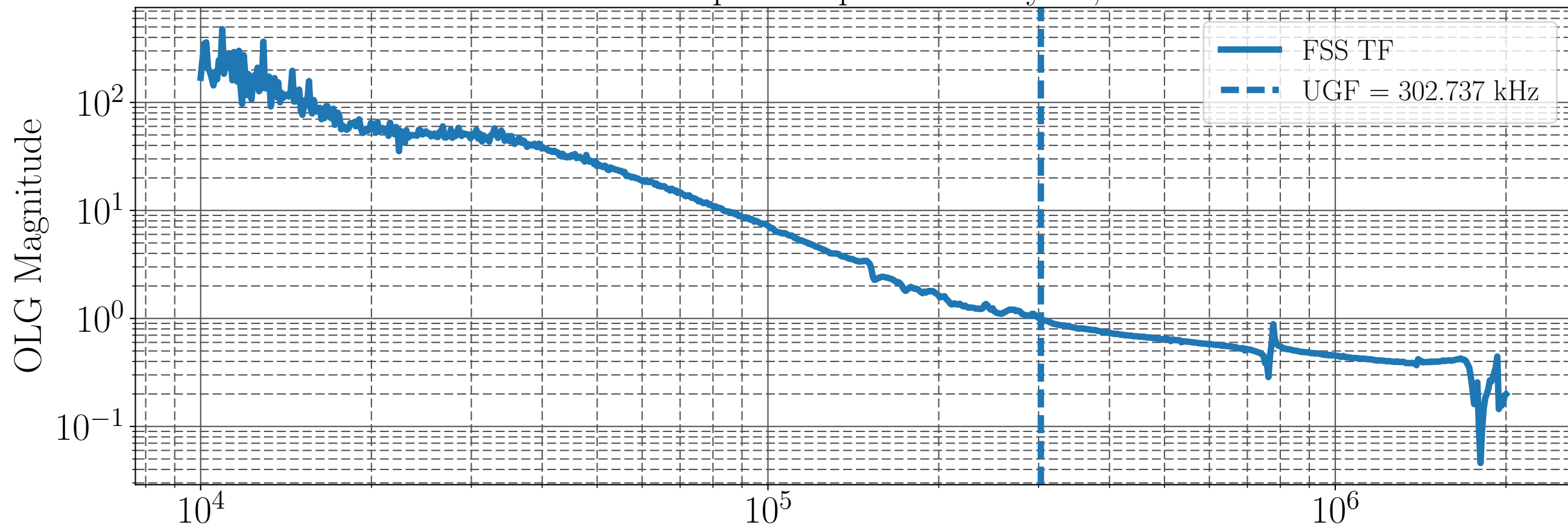
LHO FSS Open Loop Gain - July 17, 2018
