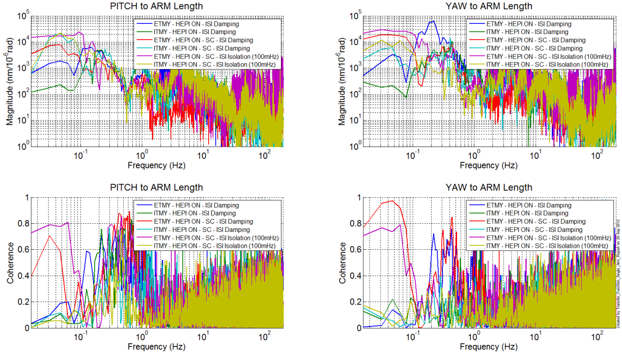
Figure 3 - Transfer function Tilt to length of the cavity
