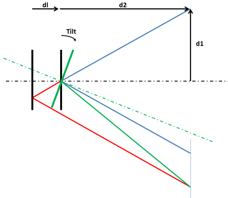
Figure 2 - Optical levers
