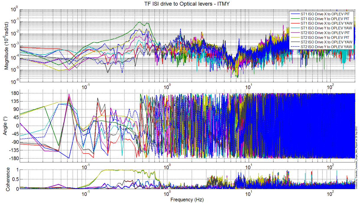
Figure 4 – Transfer functions from the Cartesian drives (X-Y) of the ISI to the optical levers – ITMY Cavity Unlocked
