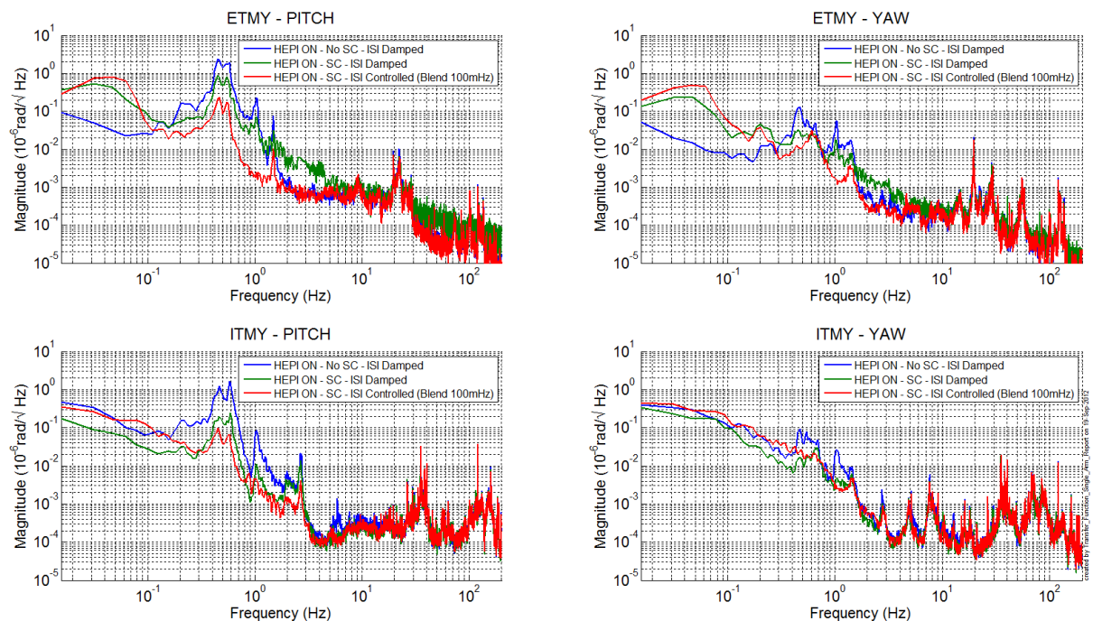
Figure 1 - ASD Optical levers
