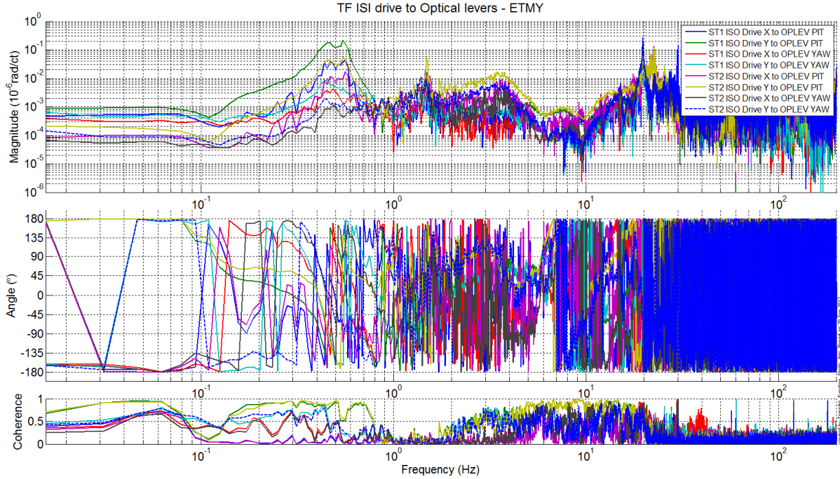
Figure 5 - Transfer functions from the Cartesian drives (X-Y) of the ISI to the optical levers – ETMY Cavity Unlocked
