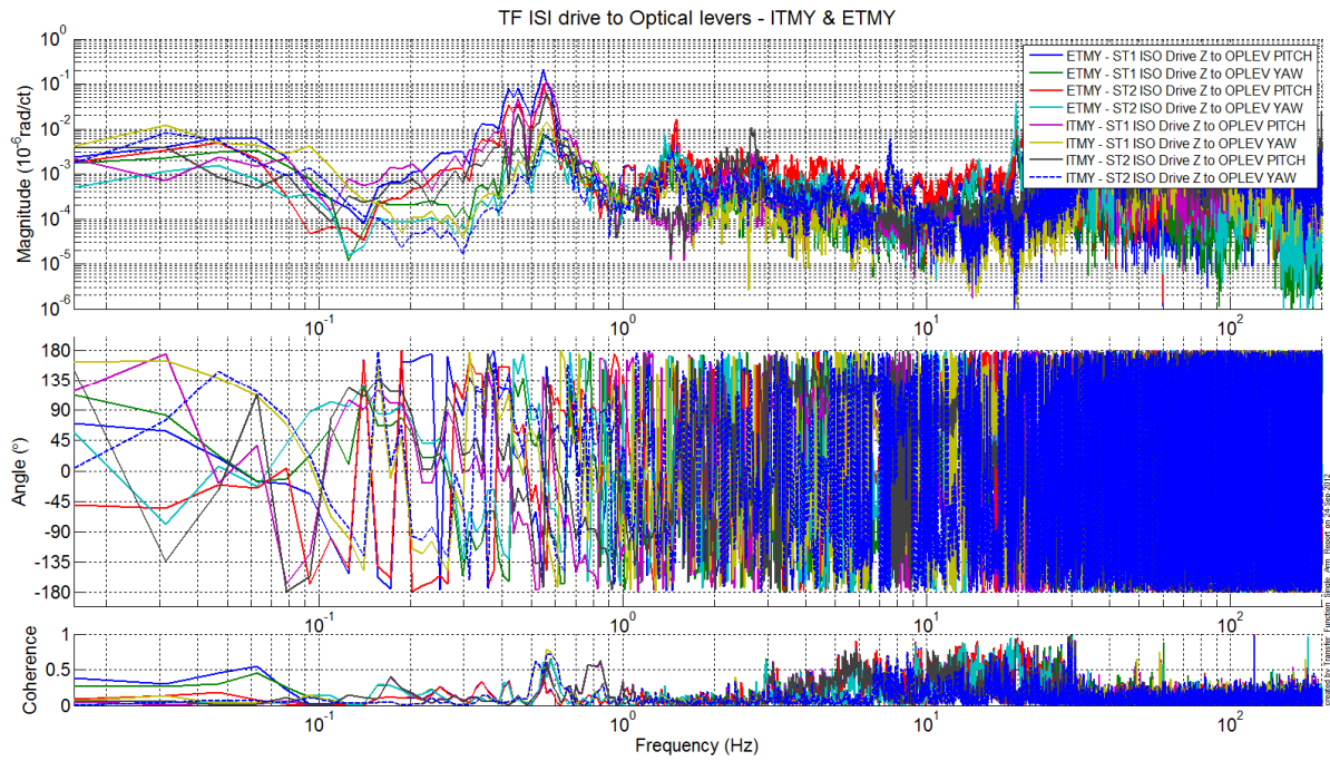
Figure 6 - Transfer functions from the Cartesian drives (Z) of the ISI to the optical levers
