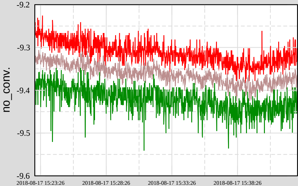
Ch 3: H1:SQZ-CLF_REFL_RF6_DEMOD_RFMON
