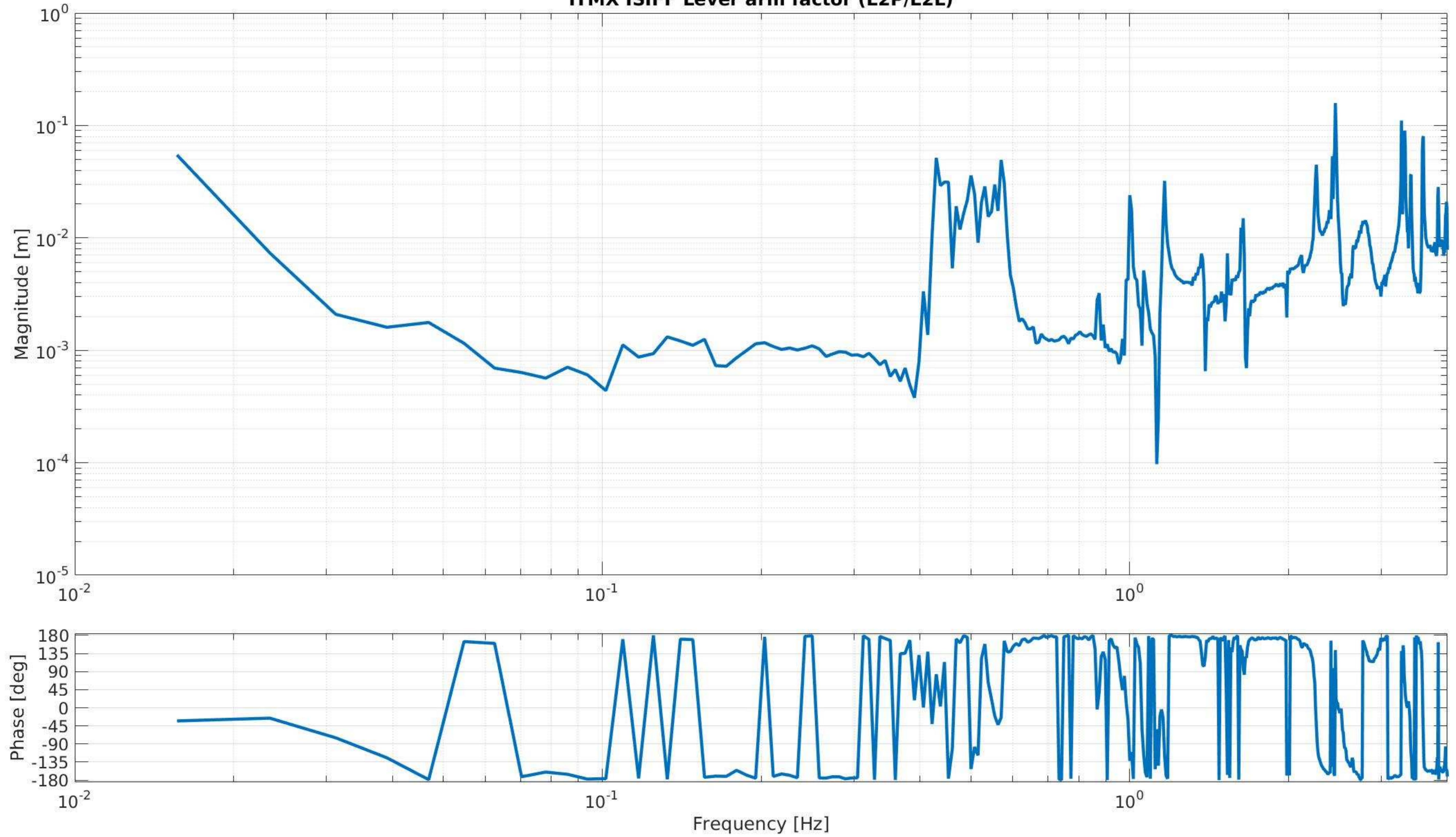
ITMX ISIFF Lever arm factor (L2P/L2L)
