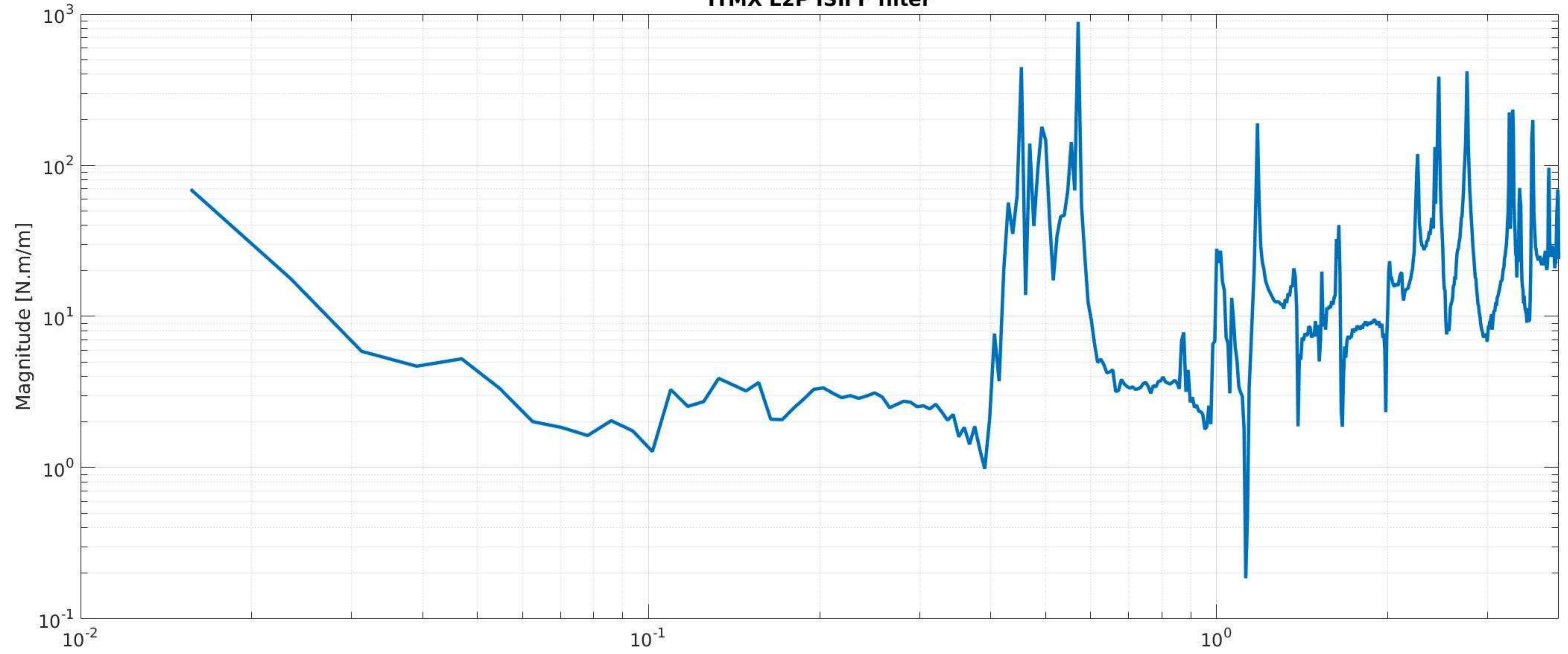
ITMX L2P ISIFF filter
