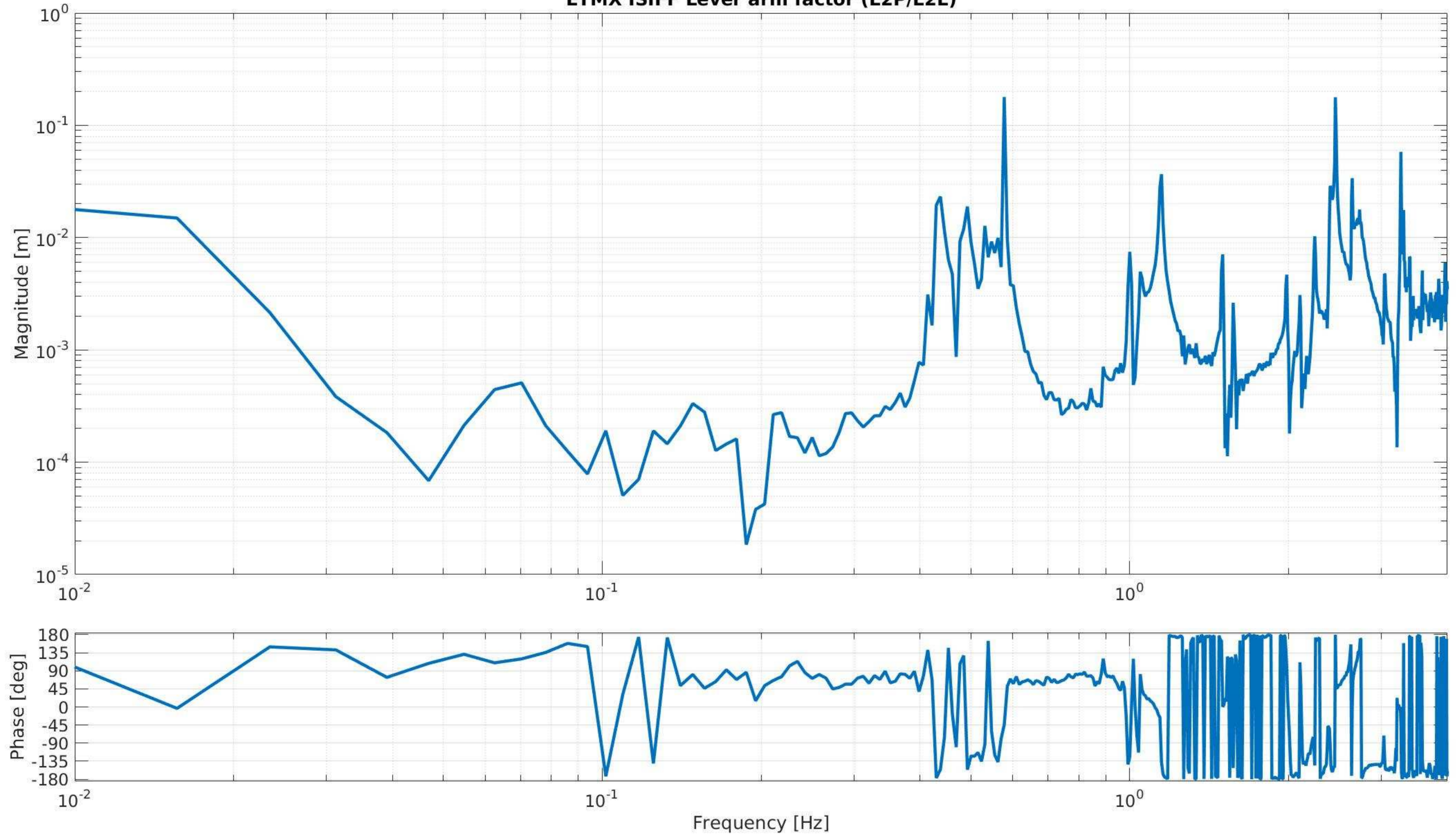
ETMX ISIFF Lever arm factor (L2P/L2L)
