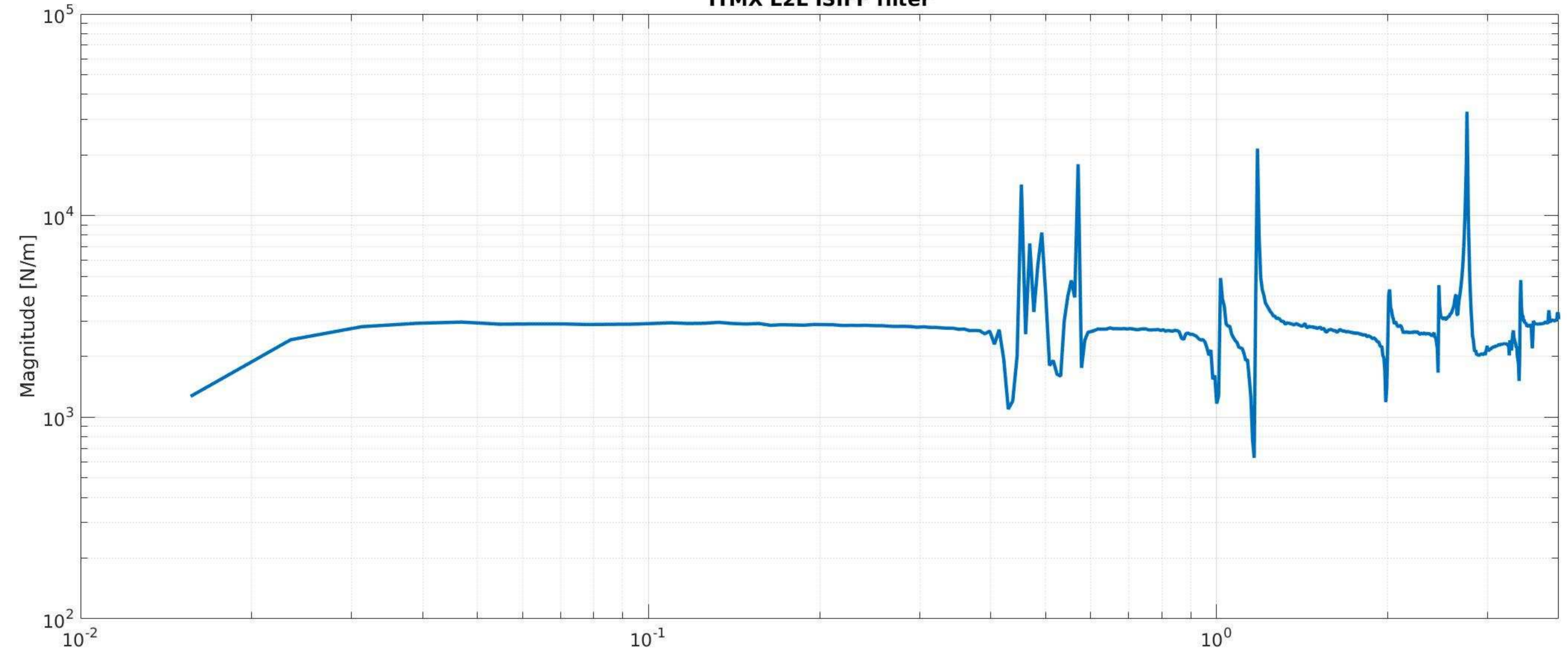
ITMX L2L ISIFF filter
