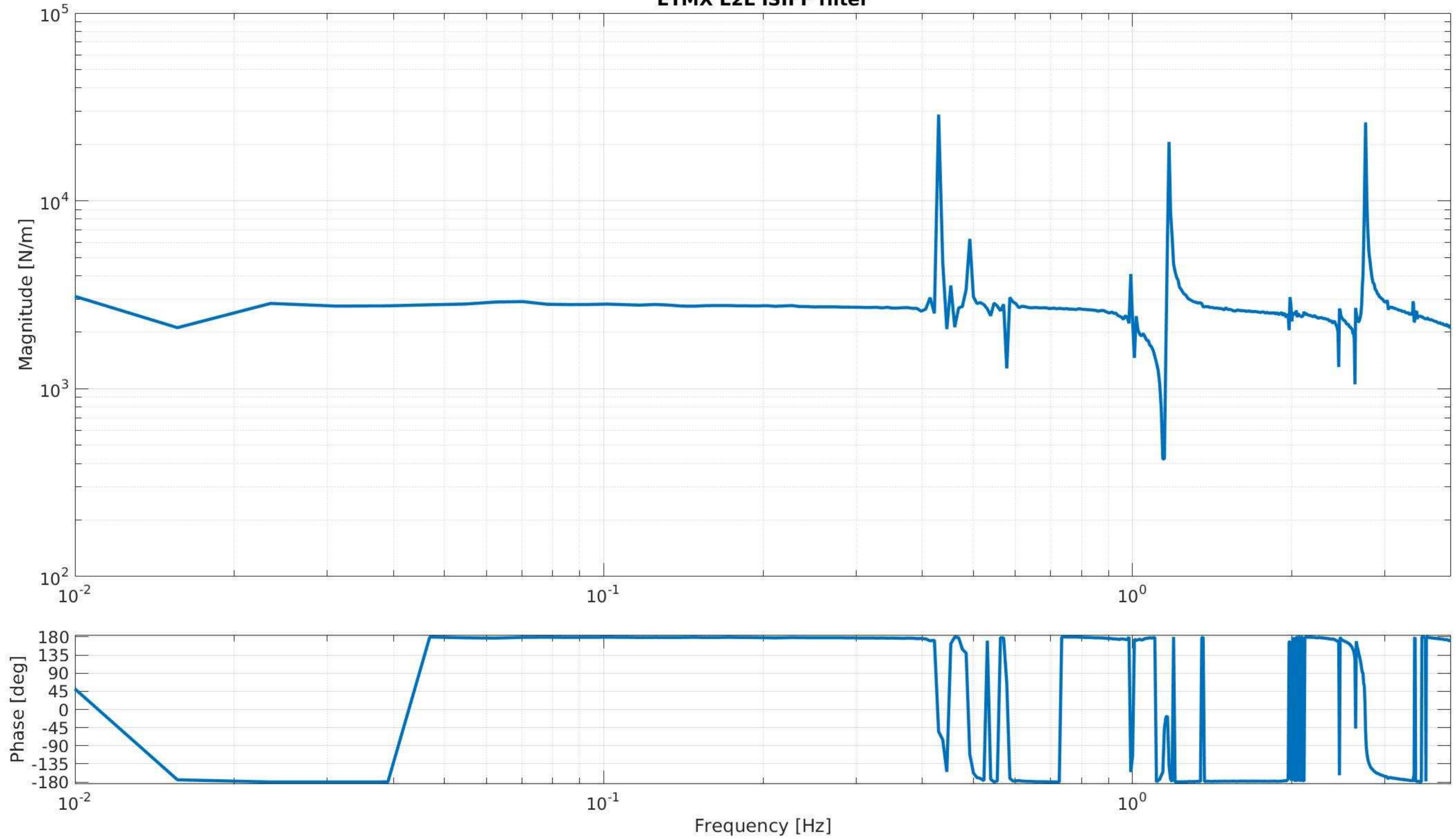
ETMX L2L ISIFF filter
