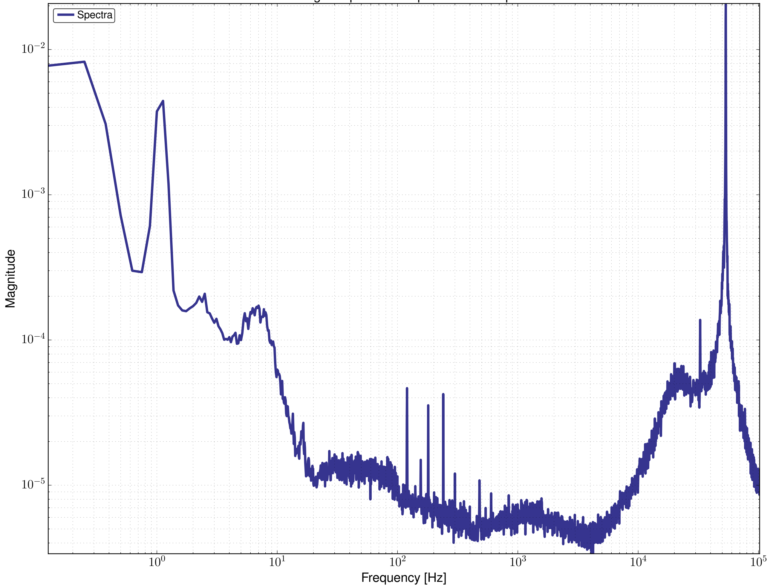
IMC Error Signal Spectrum - Input 2 watts - Sep-04-2018
