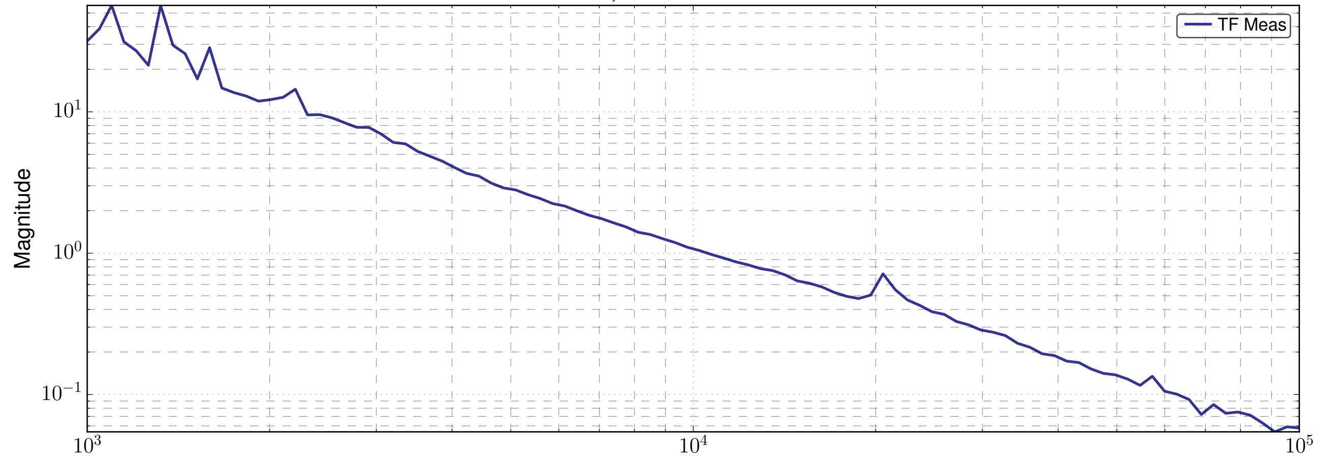
CARM OLG at 5W input power after REFL9 Phasing CARM IN1 Gain = 1 dB, SumNode Gain = -15 dB - Oct-01-2018
