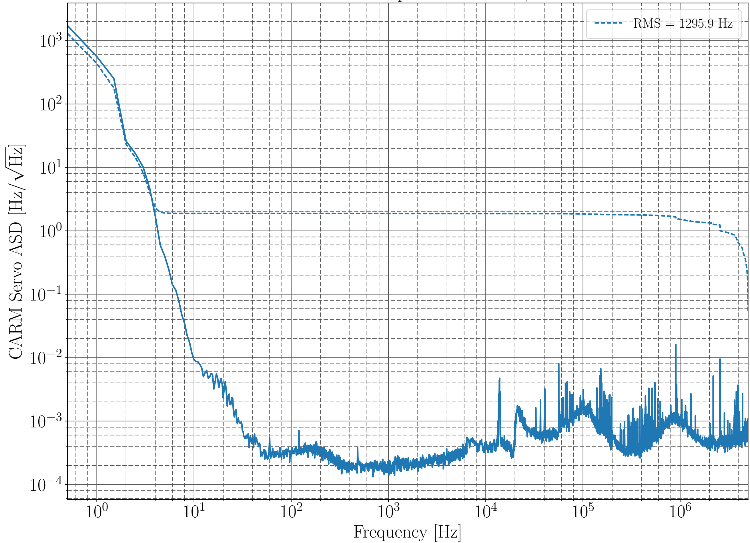
Calibrated CARM Spectrum - Oct 24, 2018
