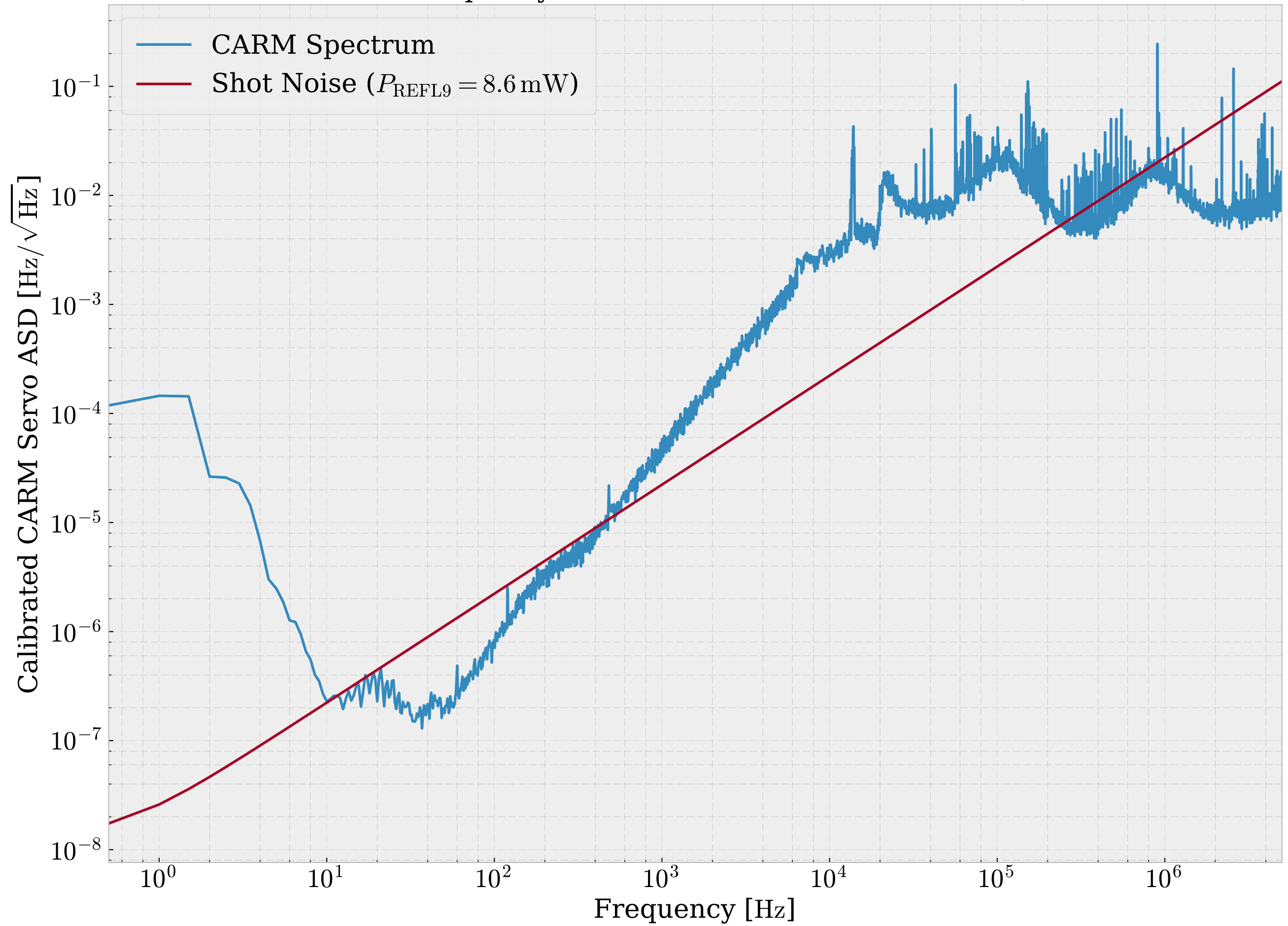
Residual Frequency Noise Incident on the IFO - Oct 30, 2018
