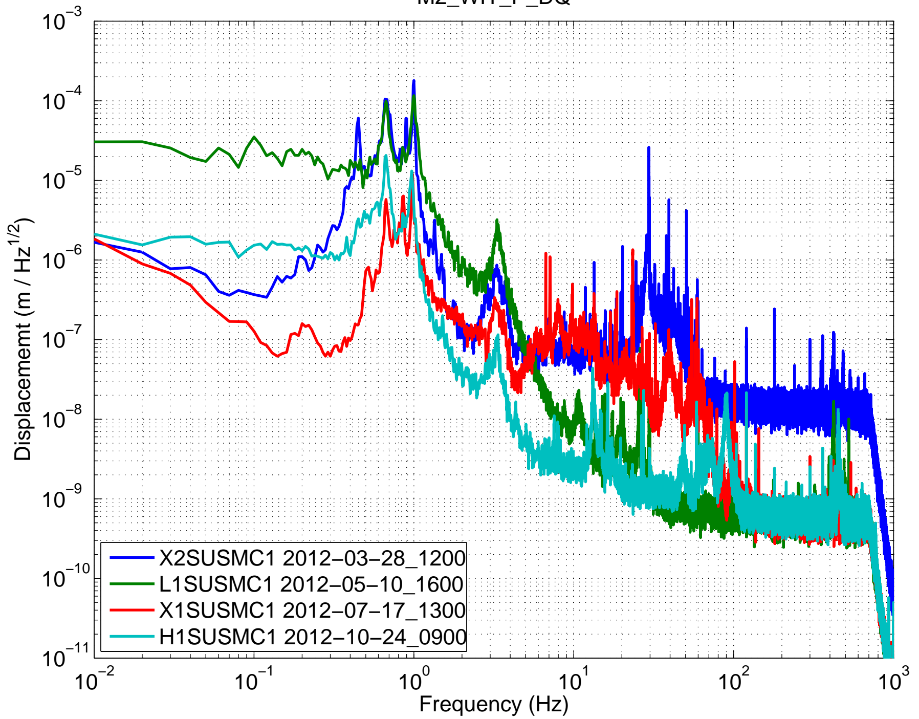
(HSTS) Amplitude Spectral Density – Damping ON M2_WIT_P_DQ
