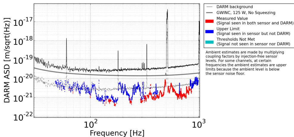
L1:IMC-WFS A I PITYAW QUADSUM - Composite Estimated Ambient (Coupling factors chosen based on loudest injection at each frequency)
