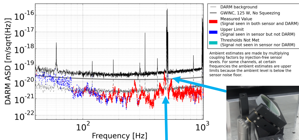
H1:IMC-WFS A DC PITYAW QUADSUM - Composite Estimated Ambient (Coupling factors chosen based on loudest injection at each frequency)
