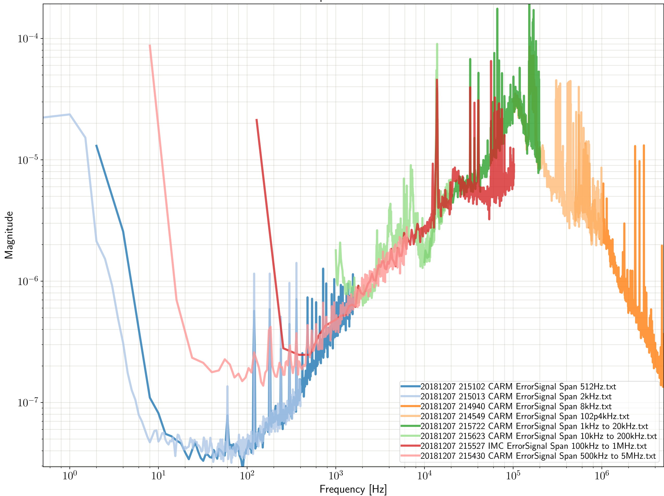
CARM Error Spectrum 20 W - Dec-07-2018
