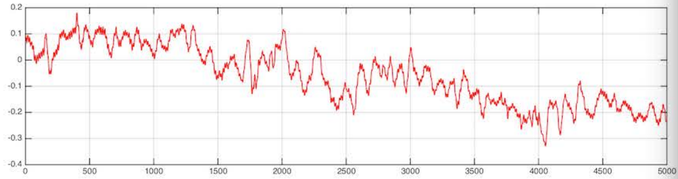
H1:IMC-WFS_A_DC_PIT_OUTPUT
