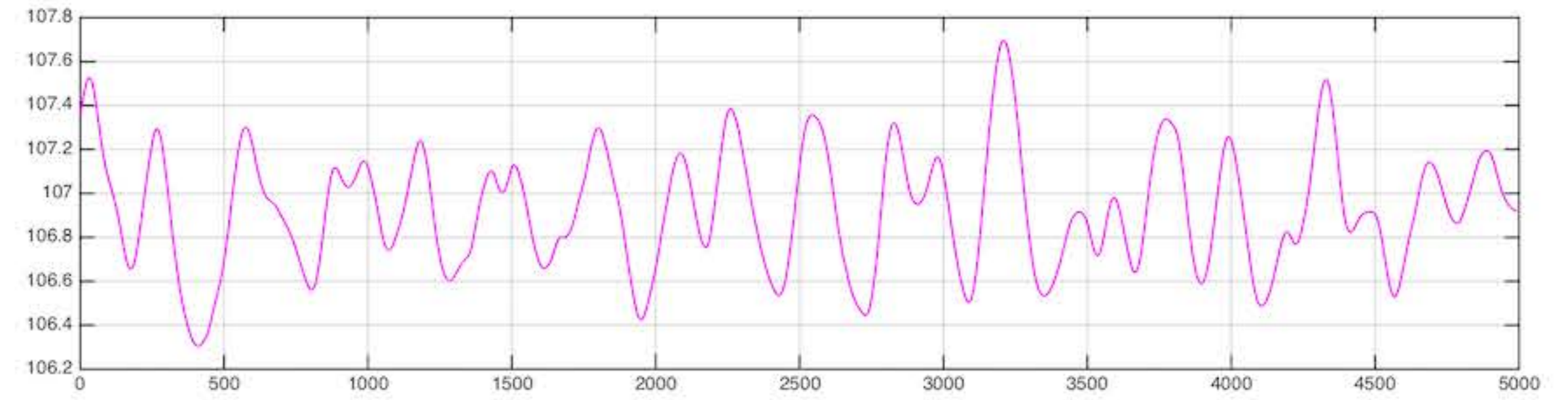
H1:PSL-PWR_PMC_TRANS_OUTPUT
