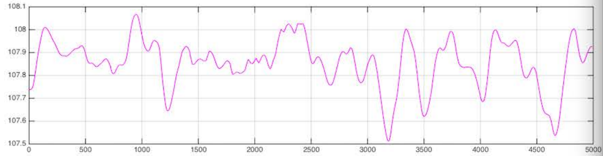
H1:PSL-PWR_PMC_TRANS_OUTPUT
