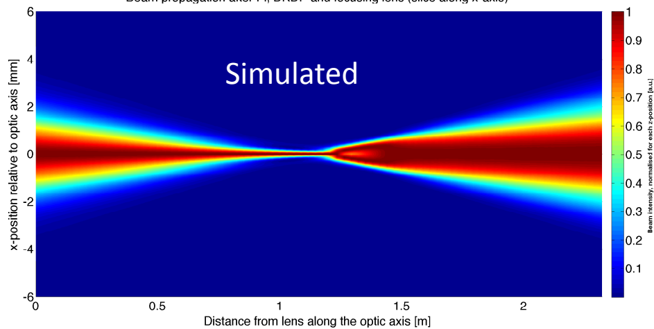
Simulated propagation (x-z plane)
