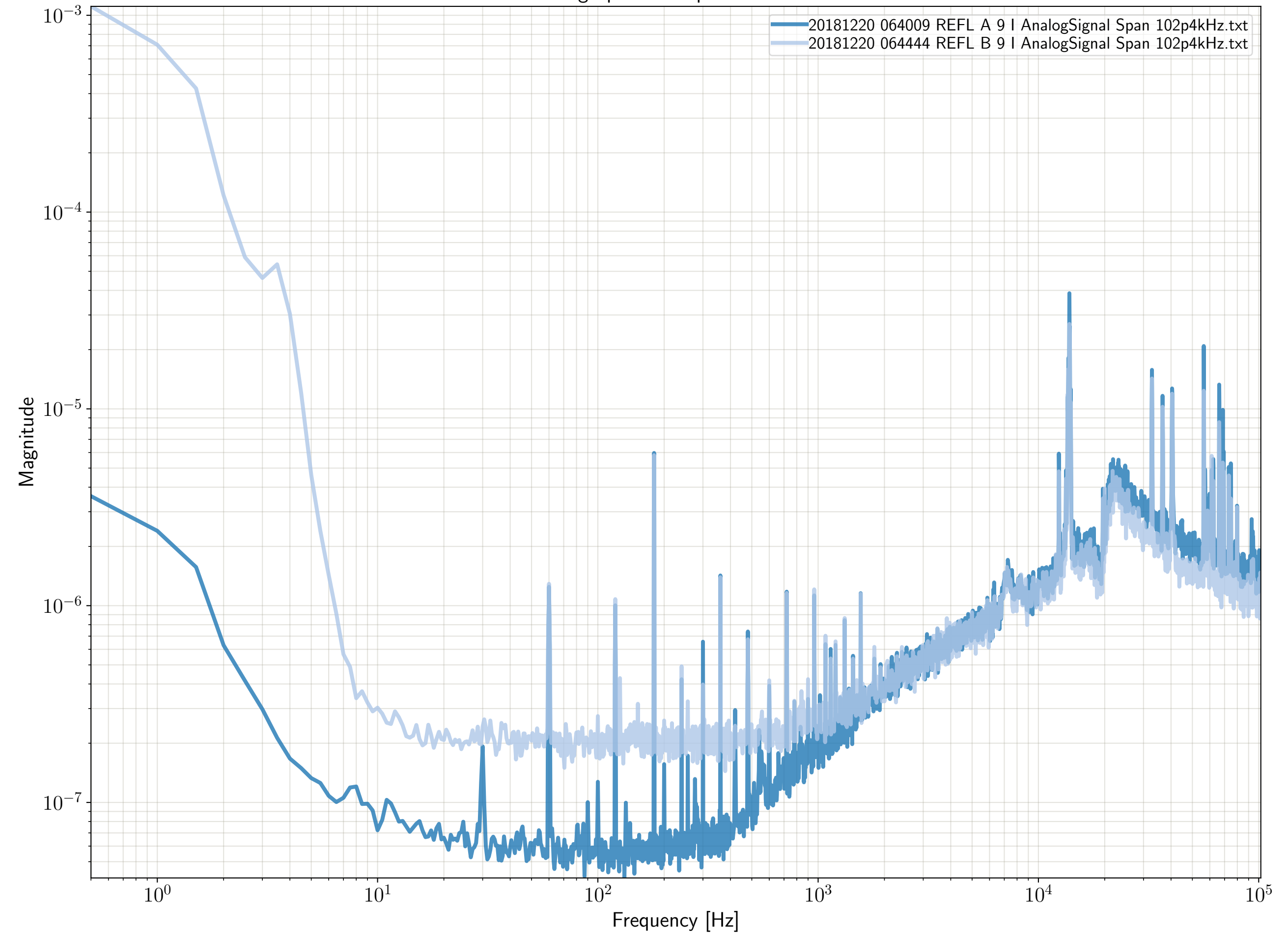
REFL A vs REFL B Analog Spectra - Input Power 20 Watts - Dec-20-2018
