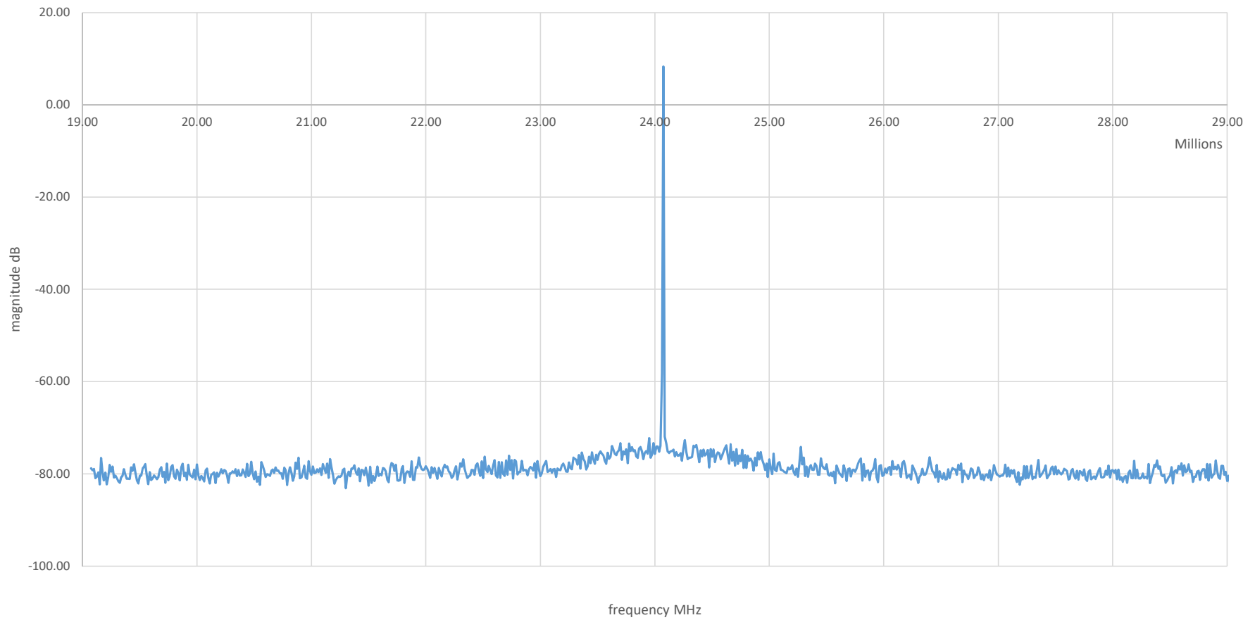
24MHz @ 300Hz Resolution Bandwidth with 6dB Attenuator
