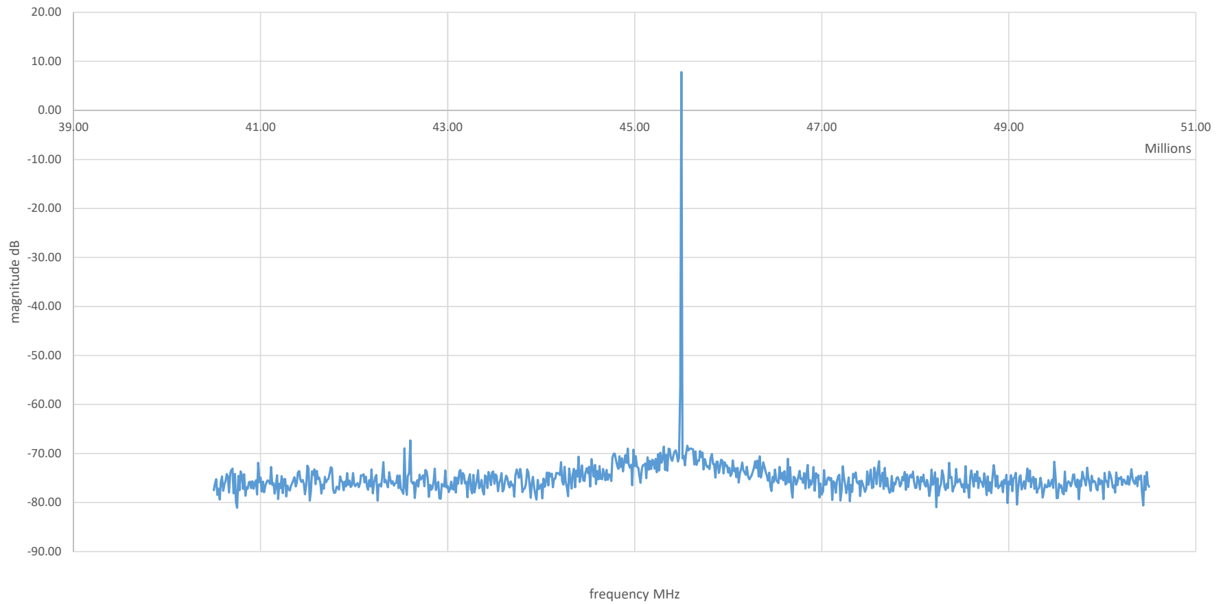
45MHz @ 300Hz Resolution Bandwidth with 6dB Attenuator
