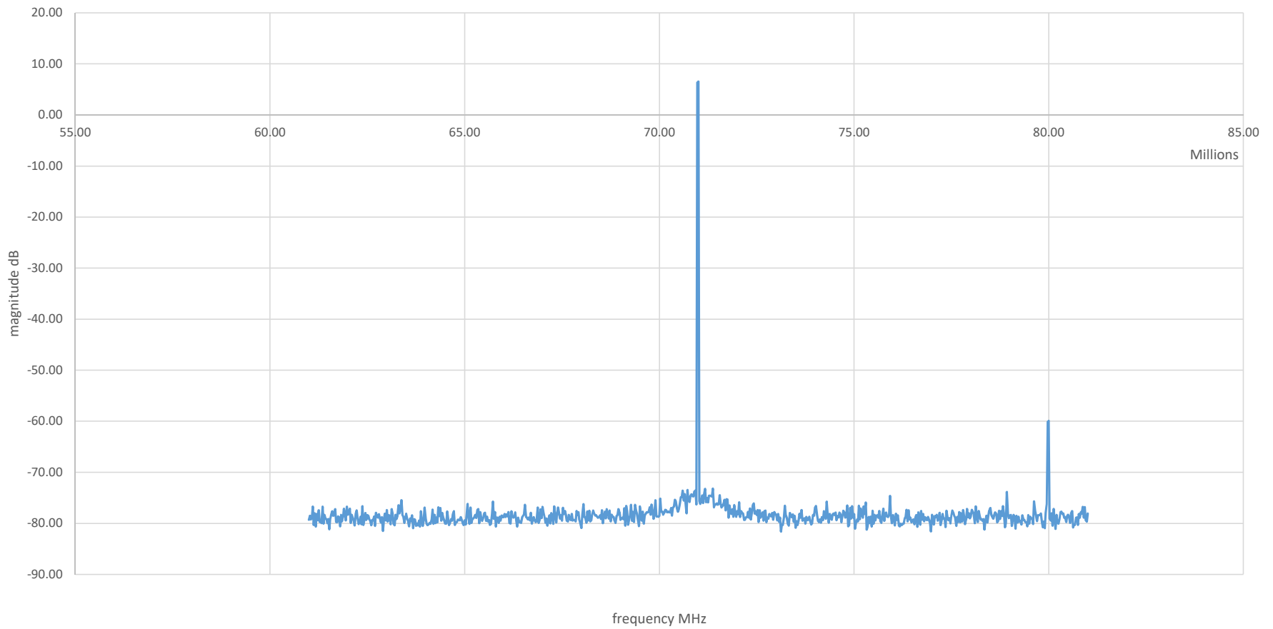
71MHz @ 300Hz Resolution Bandwidth with 6db Attenuator
