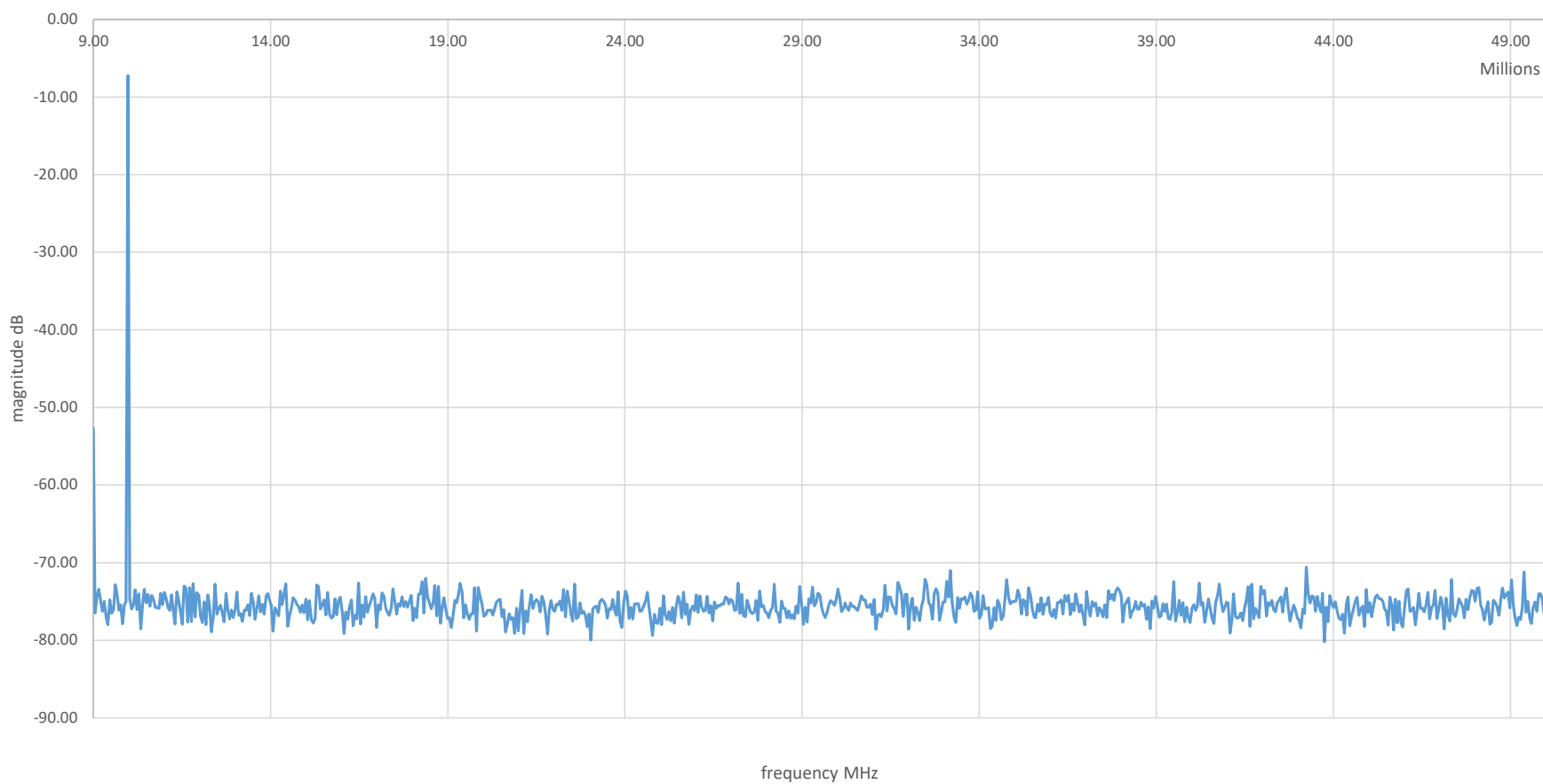
10MHz with 50MHz Span (with 10MHz LPF)
