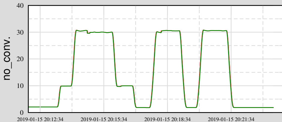
Ch 11: H1:IMC-PWR_IN_OUT16
