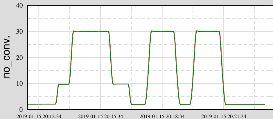
Ch 10: H1:IMC-MC2_TRANS_SUM_OUT16
