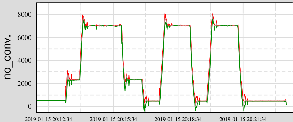
Ch 13: H1:PSL-ISS_SECONDLOOP_AC_COUPLING_DRIVE_OUT16
