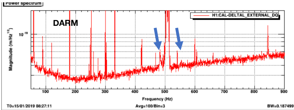
Before damping
