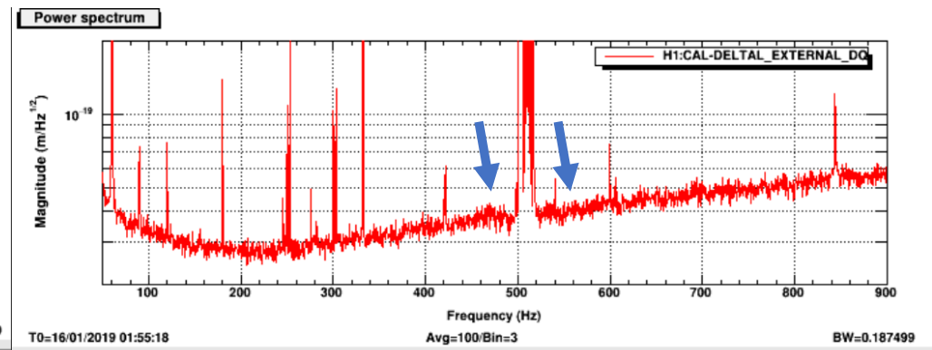
After damping
