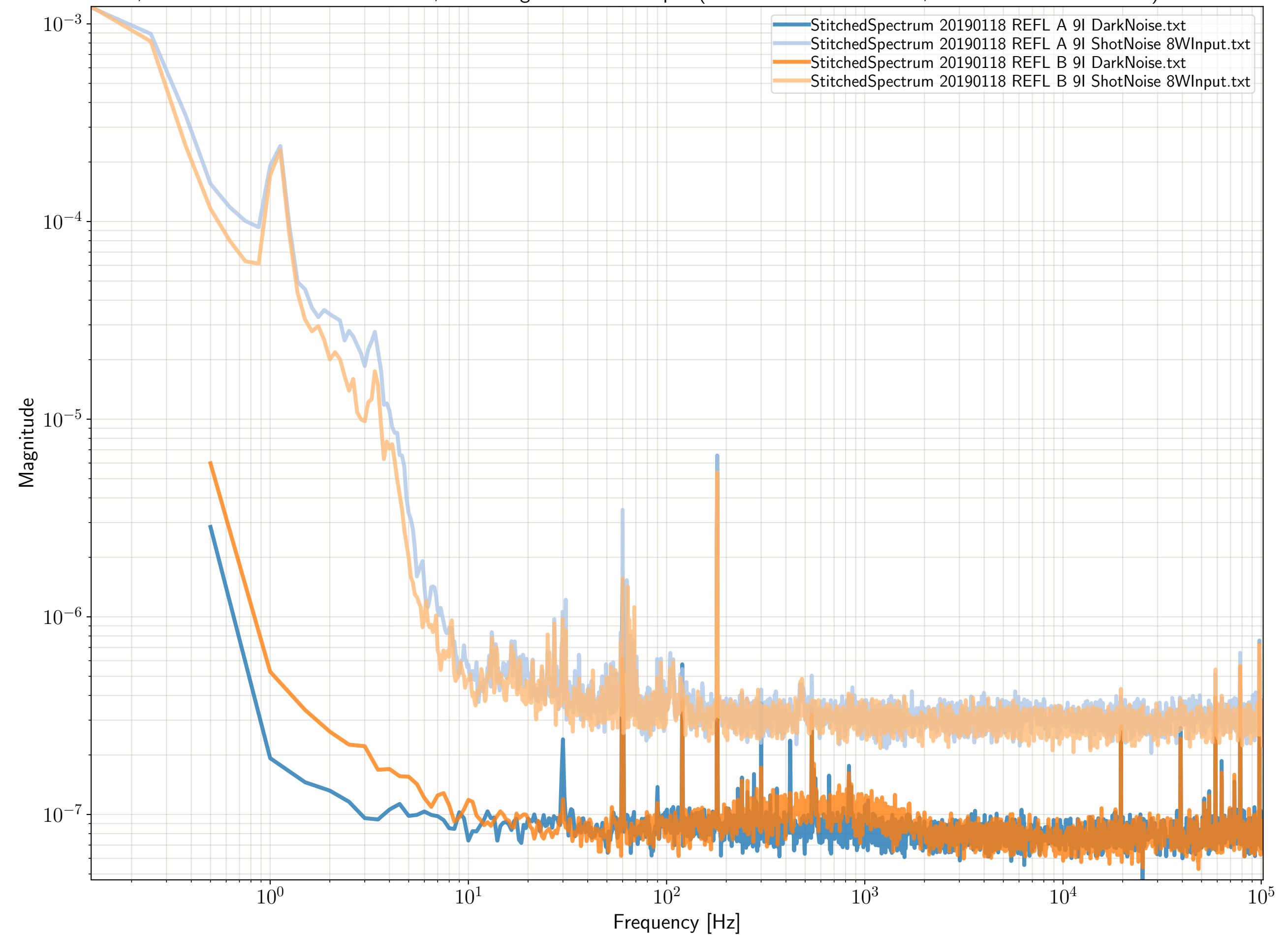
REFL A,B 9I Dark and Shot Noise No IFO, PRM Aligned with 8W Input (REFL A LF = 30.97 mW, REFL B LF = 28.52 mW) - Jan-18-2019
