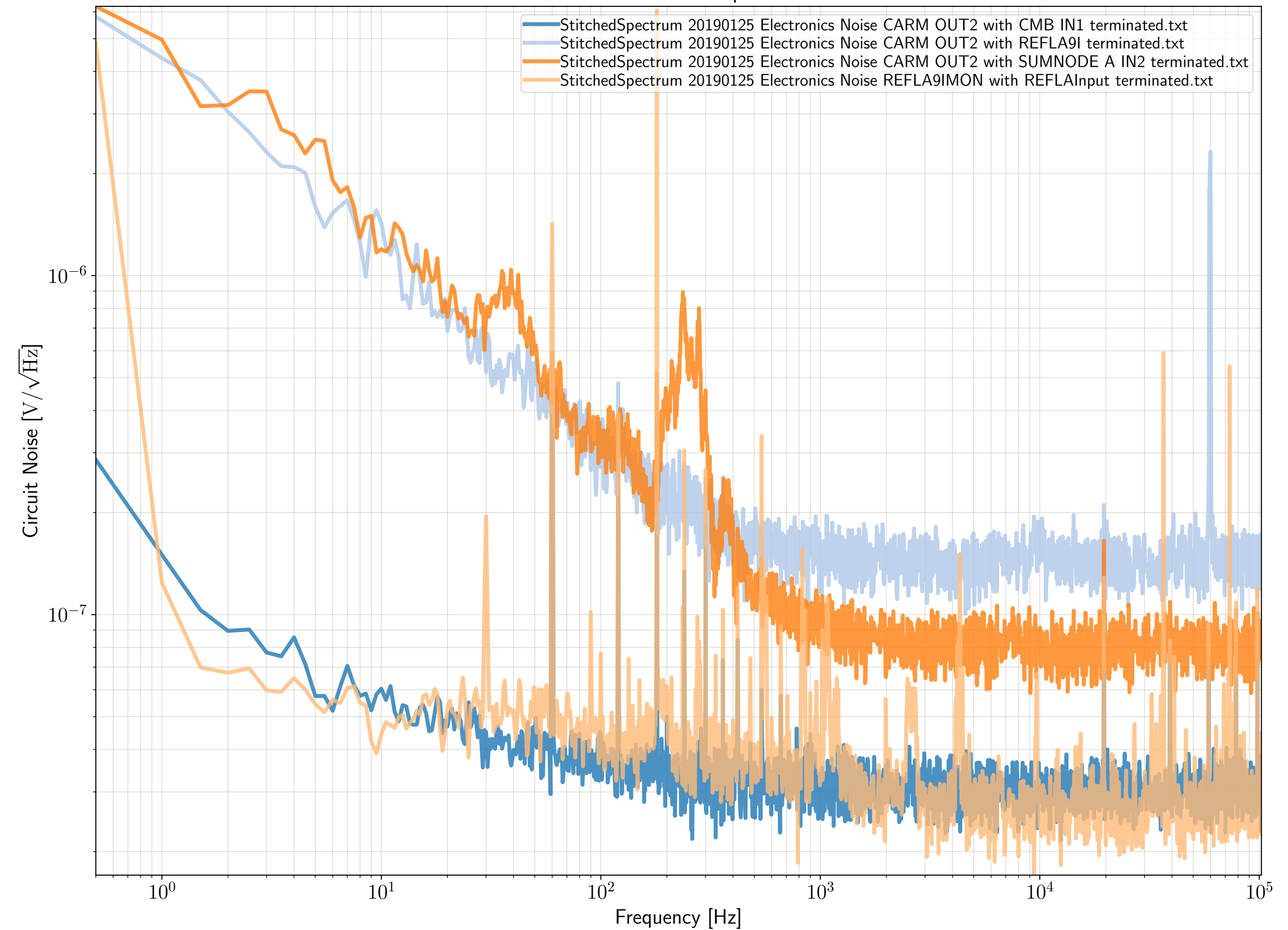
Electronics Noise in the CARM path - Jan-25-2019
