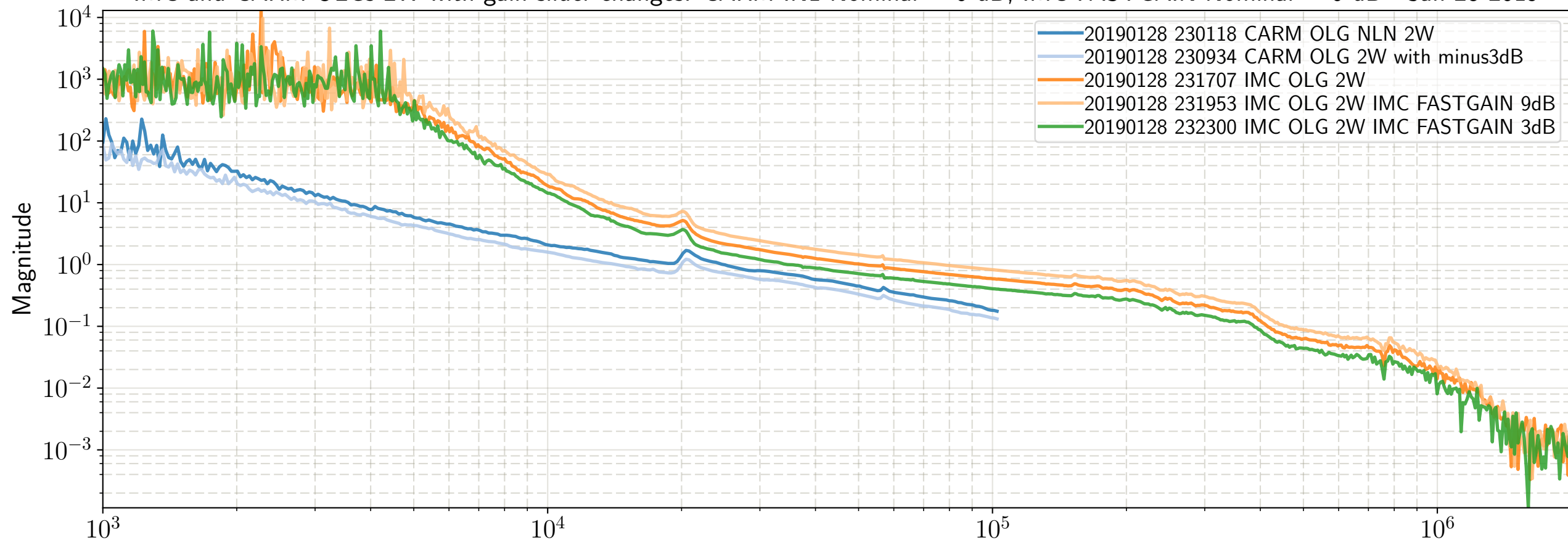
IMC and CARM OLGs 2W with gain slider changes: CARM IN1 Nominal = 0 dB, IMC FASTGAIN Nominal = 6 dB - Jan-28-2019
