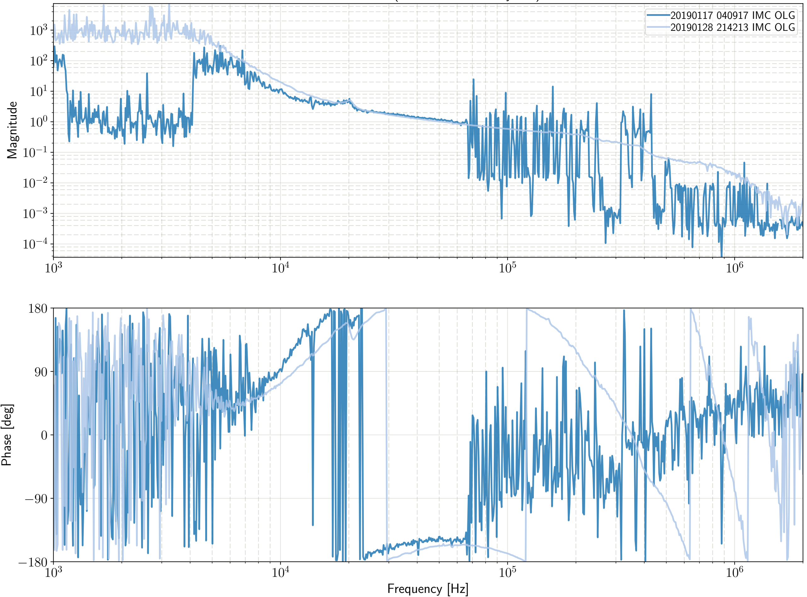
IMC OLG at 30 W and 2 W (2 W is the non noisy one) - Jan-28-2019
