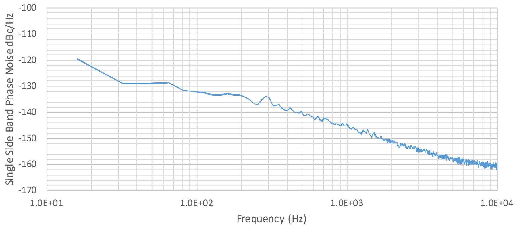
CLF VCO Phase Noise [203.125 MHz] cf. spec on LIGO-E1700010
