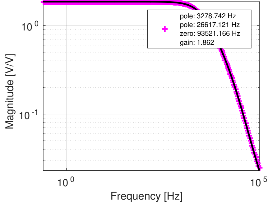
ETMY ESD LVLN driver: URnoLP (measured: 2019-02-03)
