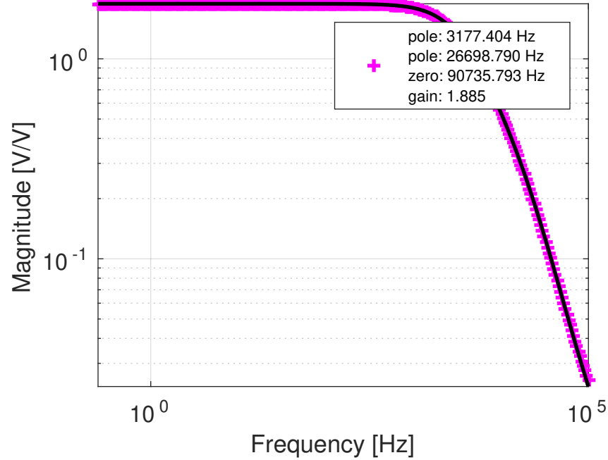
ETMY ESD LVLN driver: LLnoLP (measured: 2019-02-03)
