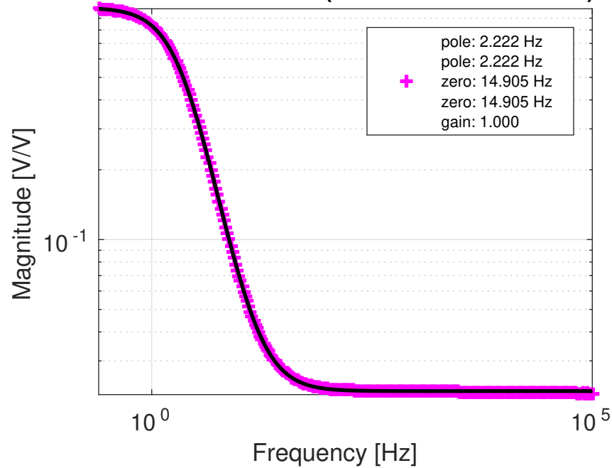
ETMY ESD LVLN driver: UR (measured: 2019-02-03)
