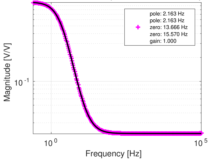
ETMY ESD LVLN driver: LL (measured: 2019-02-03)
