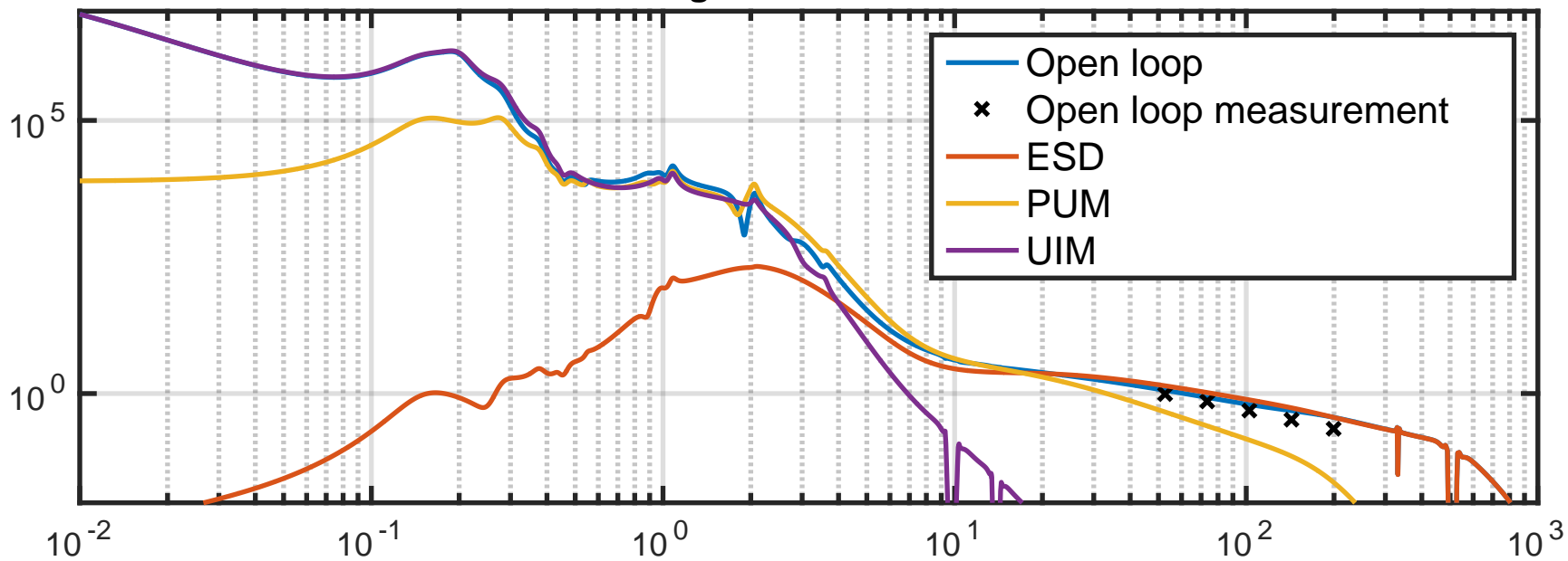
DARM gain distribution
