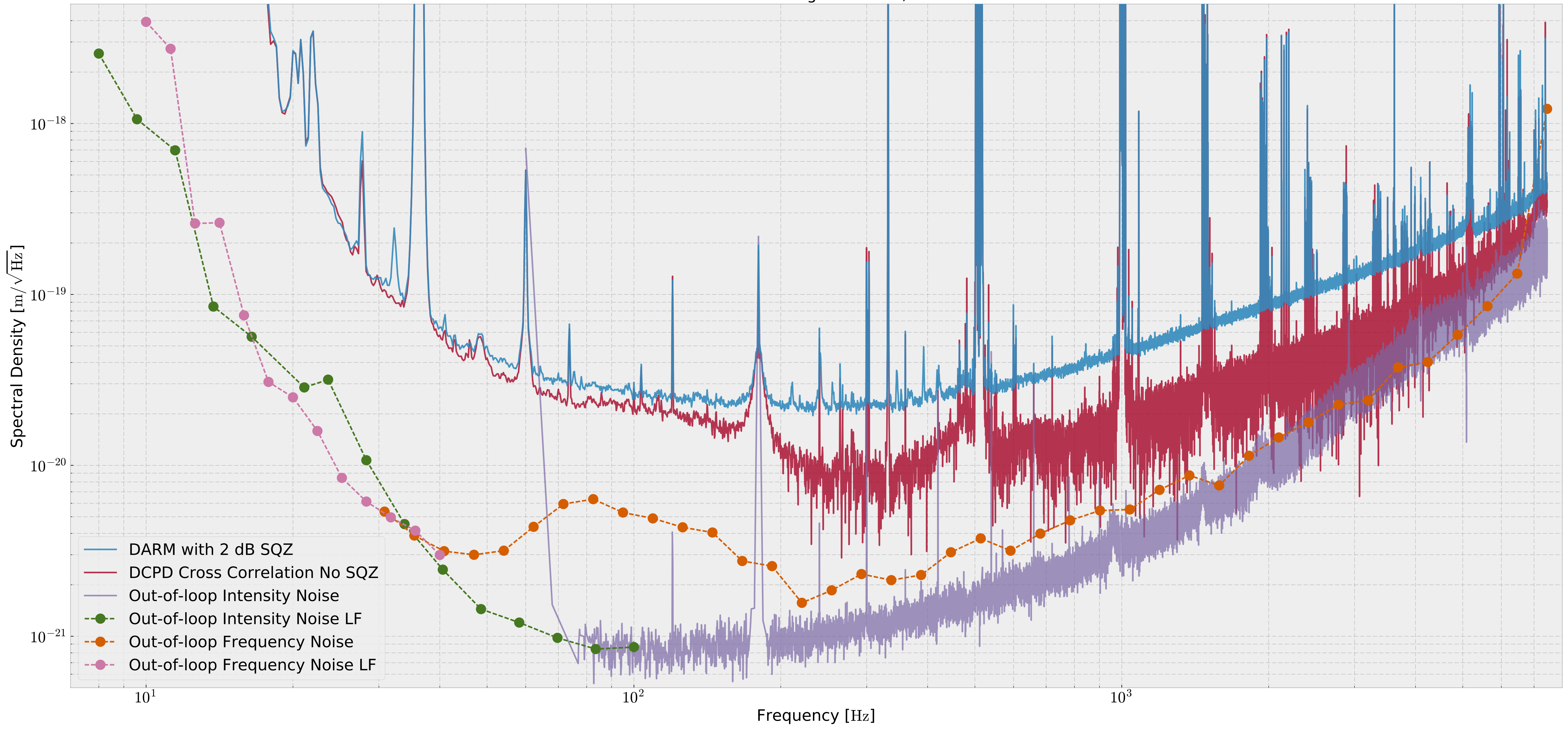
DARM Noisebudget - Feb 20, 2019
