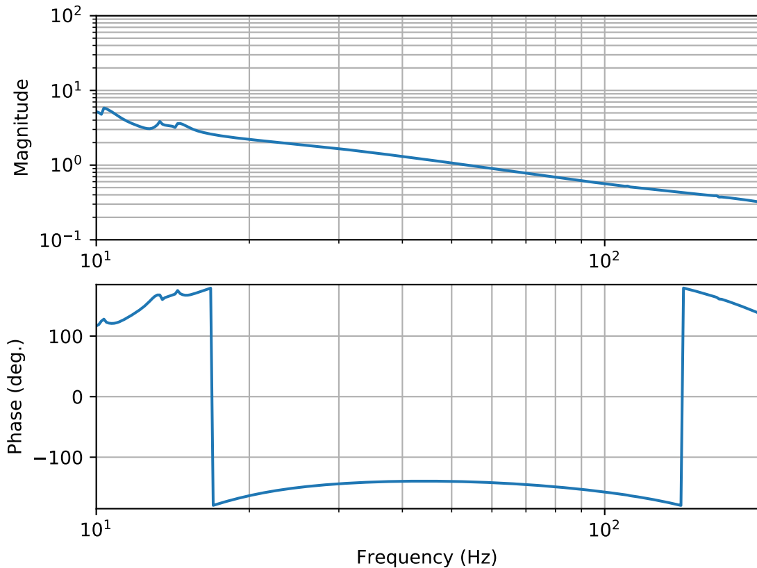
H1 open loop gain zoom
