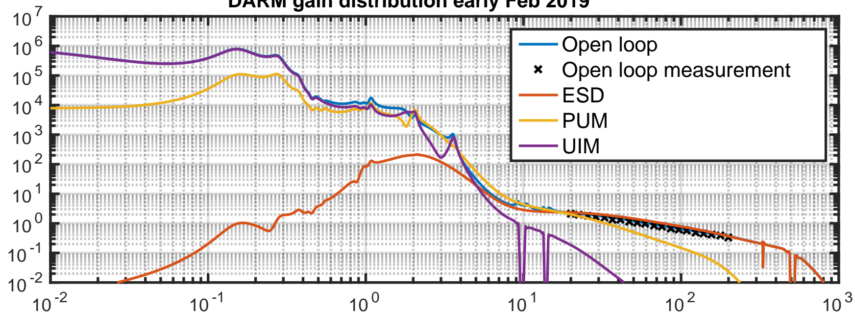
DARM gain distribution early Feb 2019
