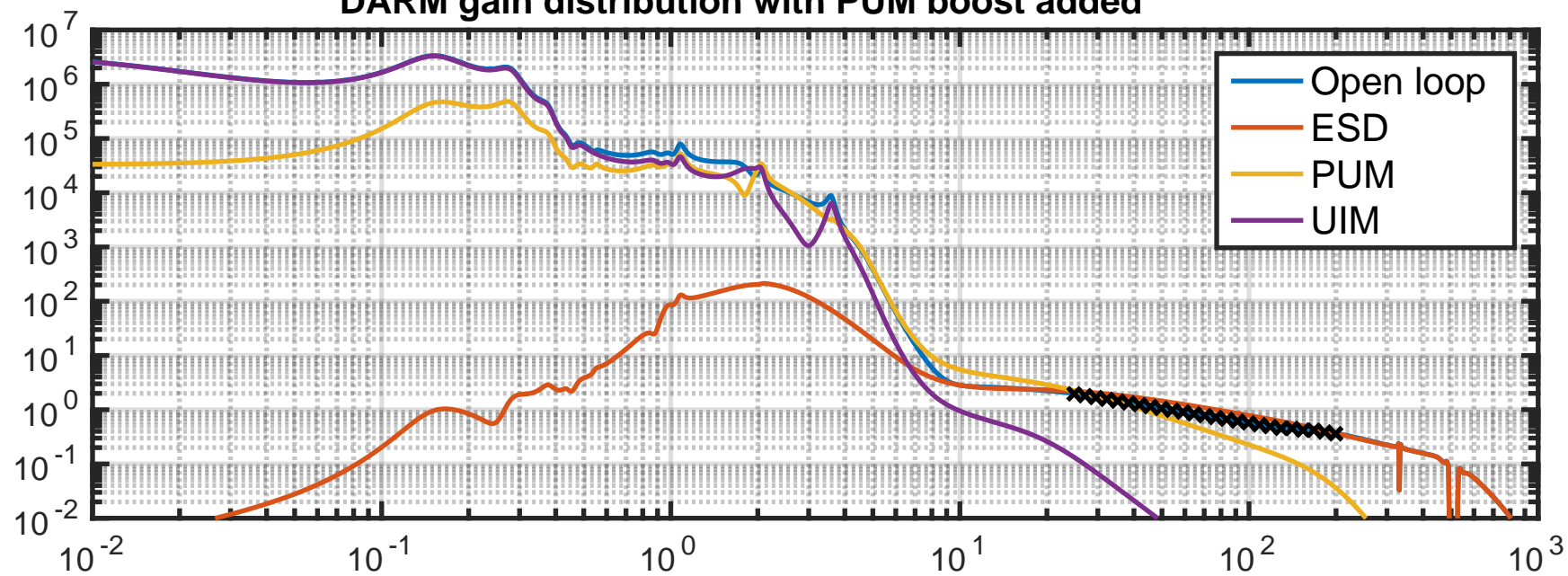
DARM gain distribution with PUM boost added
