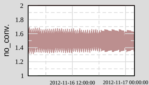
Ch 1: H0:PEM-LVEA_DST1_MODE
