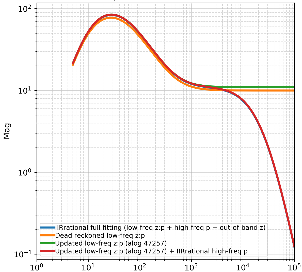
OMC TF comparison, FM1FM2FM3 or 3 filt, 4.99V DC
