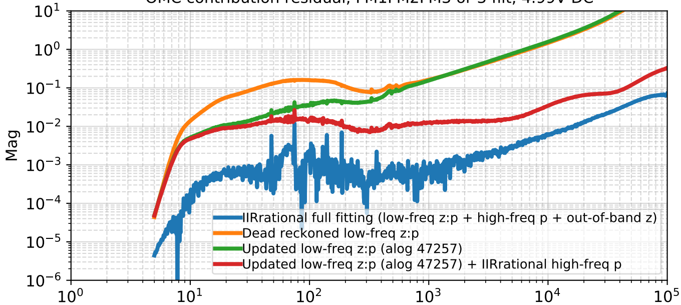
OMC contribution residual, FM1FM2FM3 or 3 filt, 4.99V DC
