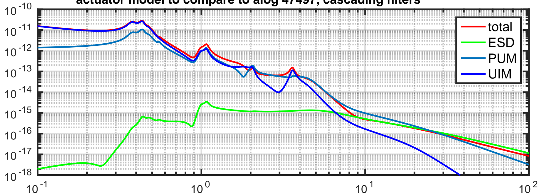
actuator model to compare to alog 47497, cascading filters
