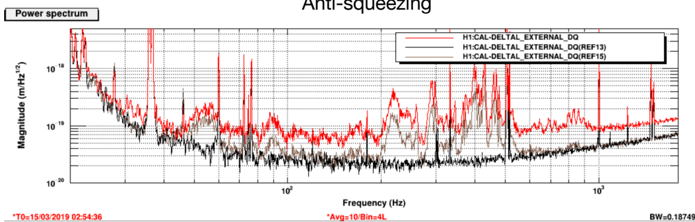
Anti-squeezing
