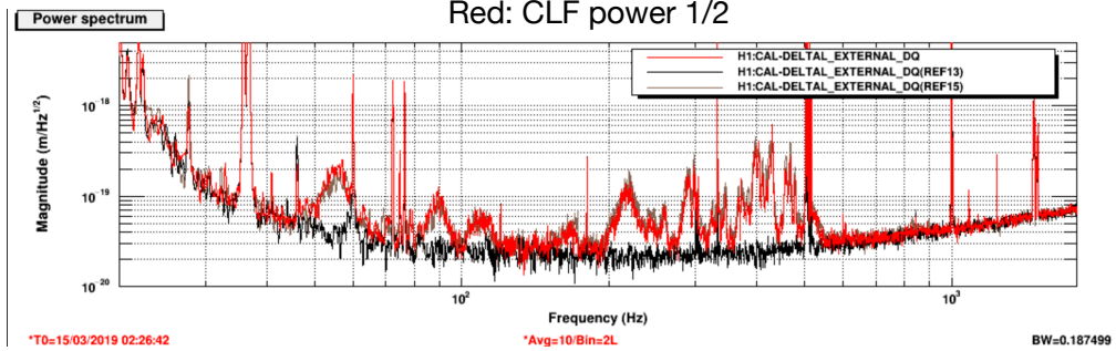
Anti-squeezing
