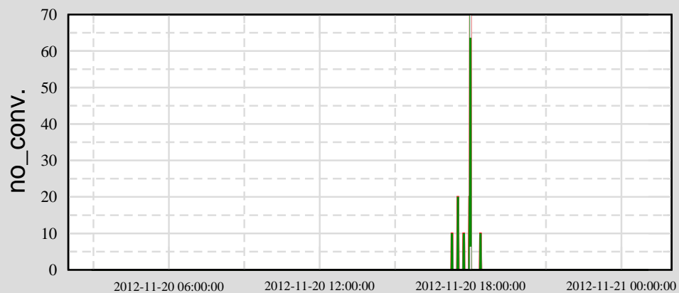
Ch 13: H0:PEM-LAB_DST1_5
