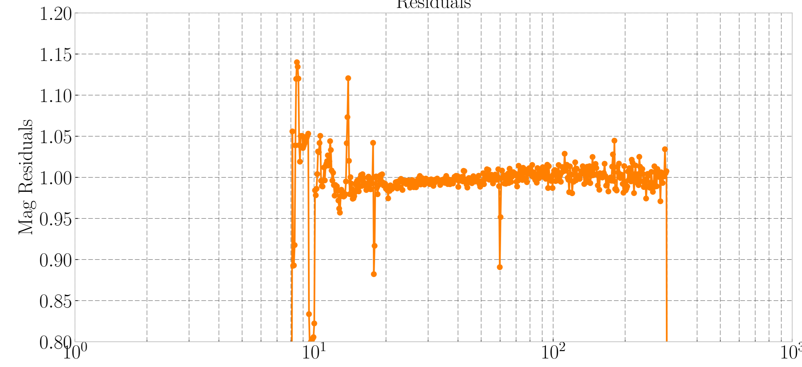
Residuals
