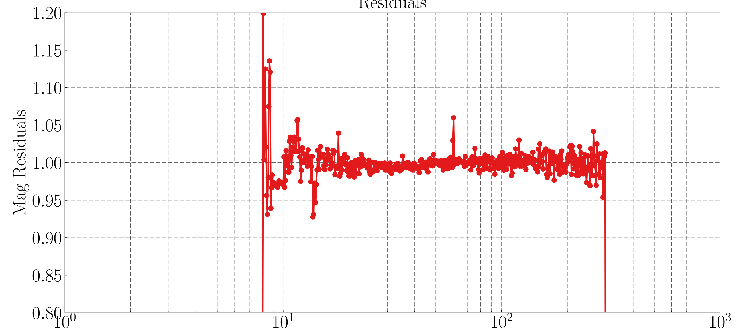
Residuals
