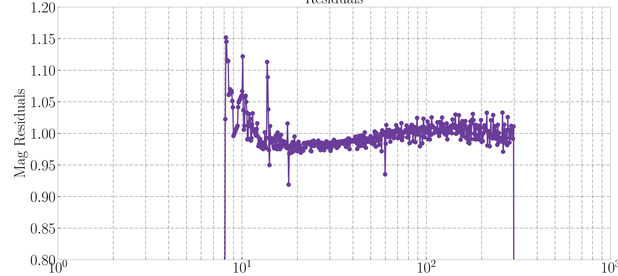
Residuals
