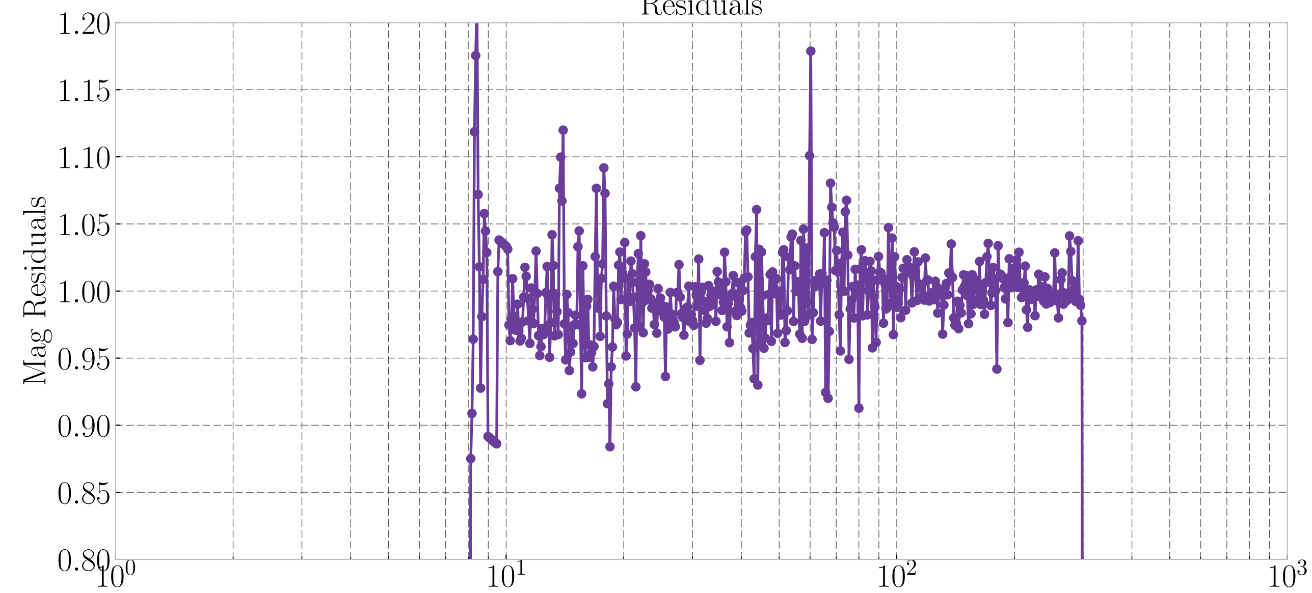
Residuals
