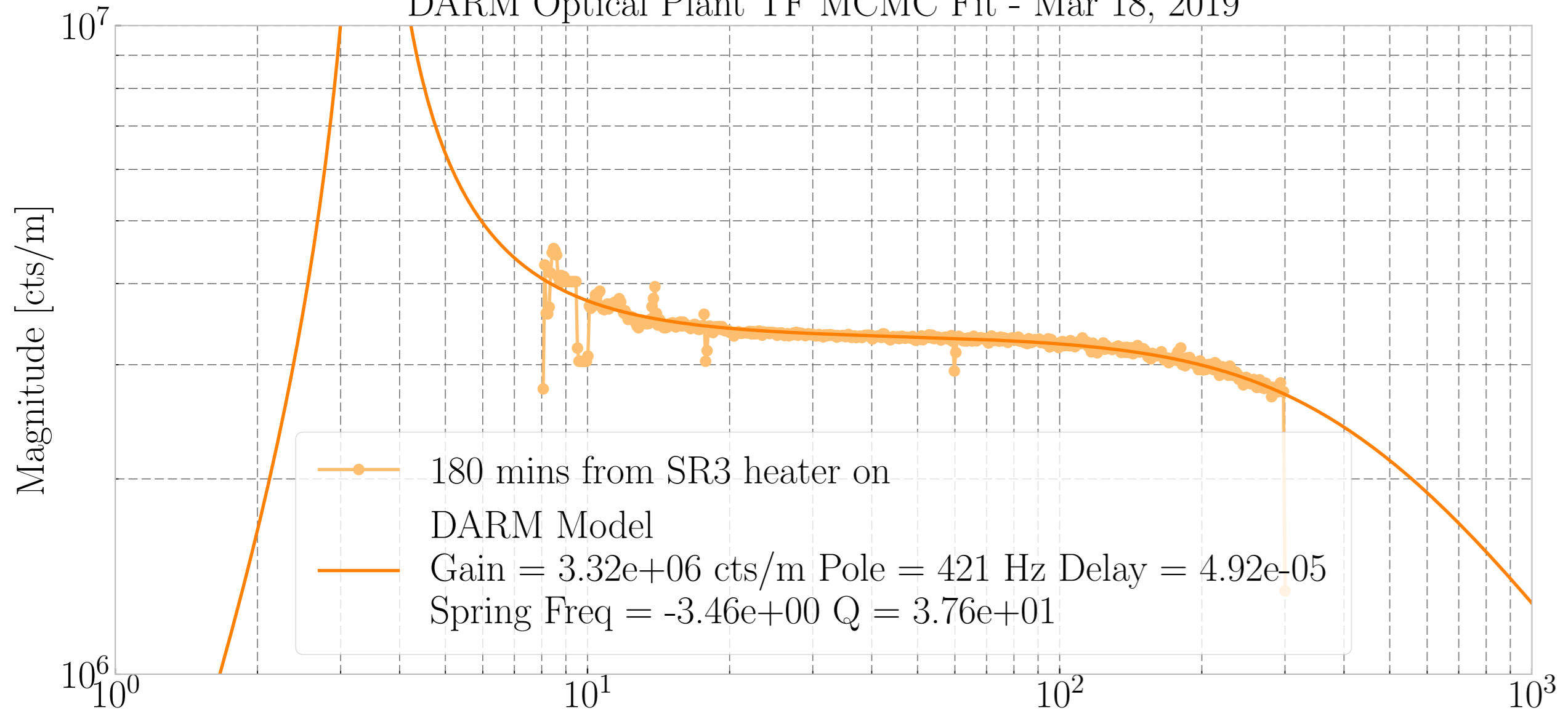
DARM Optical Plant TF MCMC Fit - Mar 18, 2019
