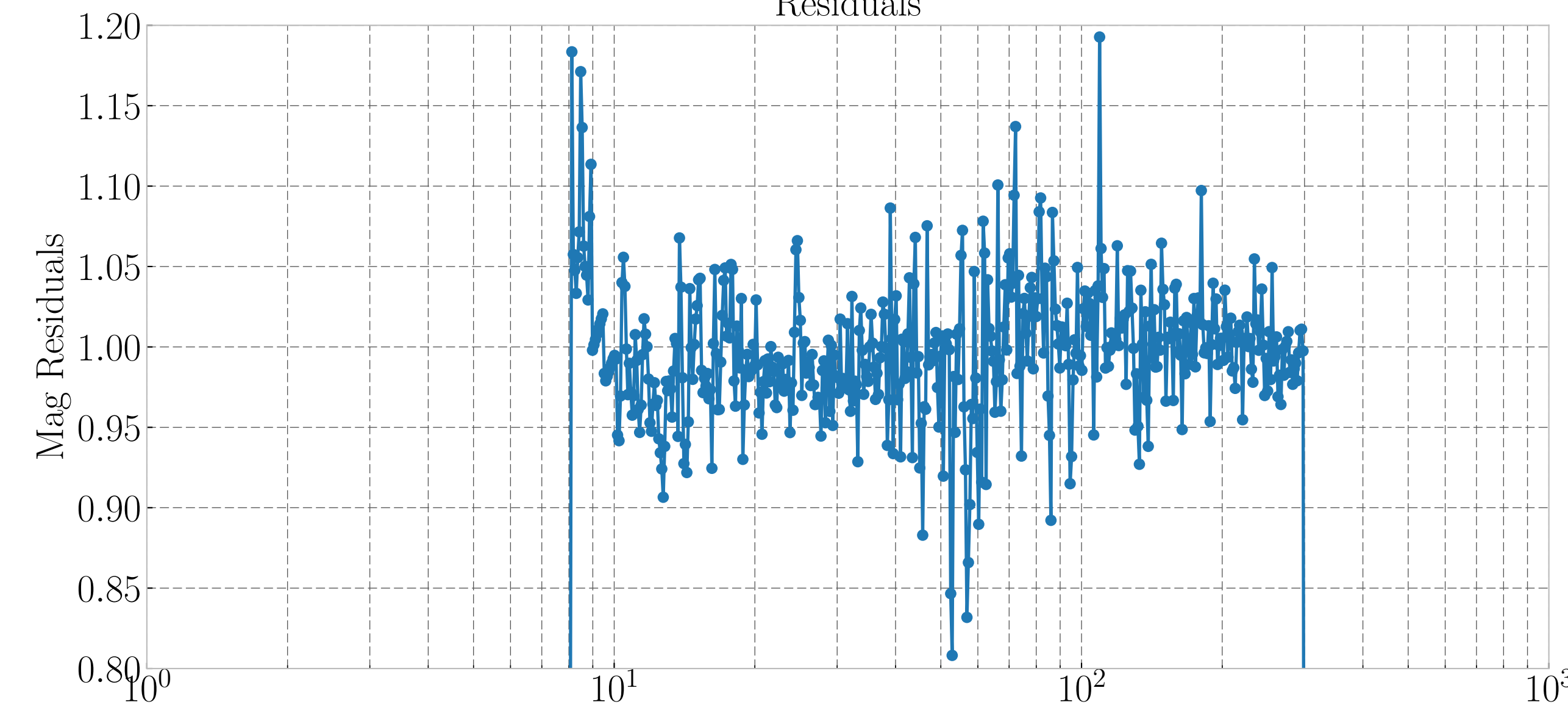
Residuals
