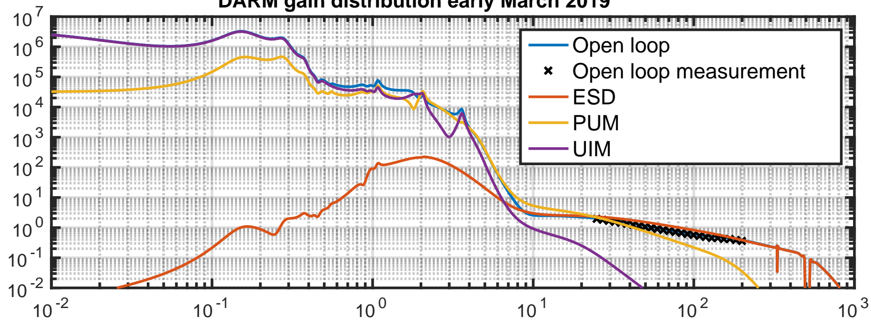
DARM gain distribution early March 2019
