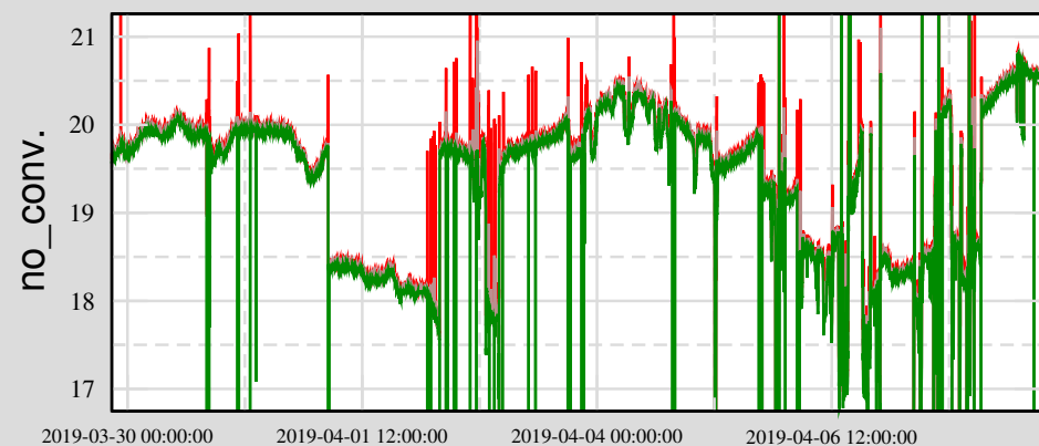
Ch 8: H1:SQZ-SHG_PWR_AOM_OUTMON
