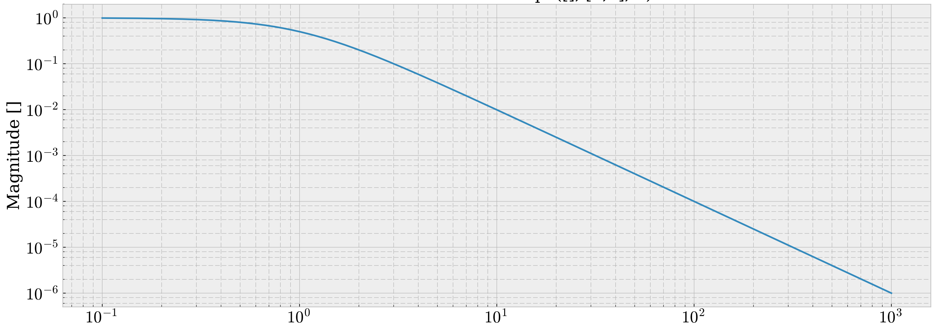
PCAL Calibration TF: \text{zpk}([], [1,1], 1)
