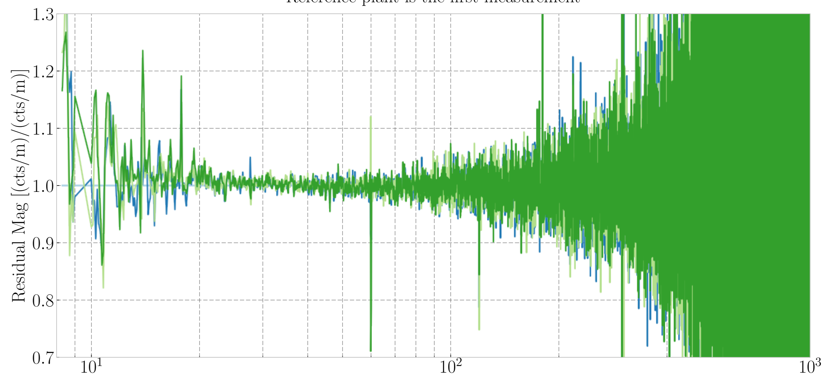
DARM Optical Plant Residuals - April 12, 2019 Reference plant is the first measurement
