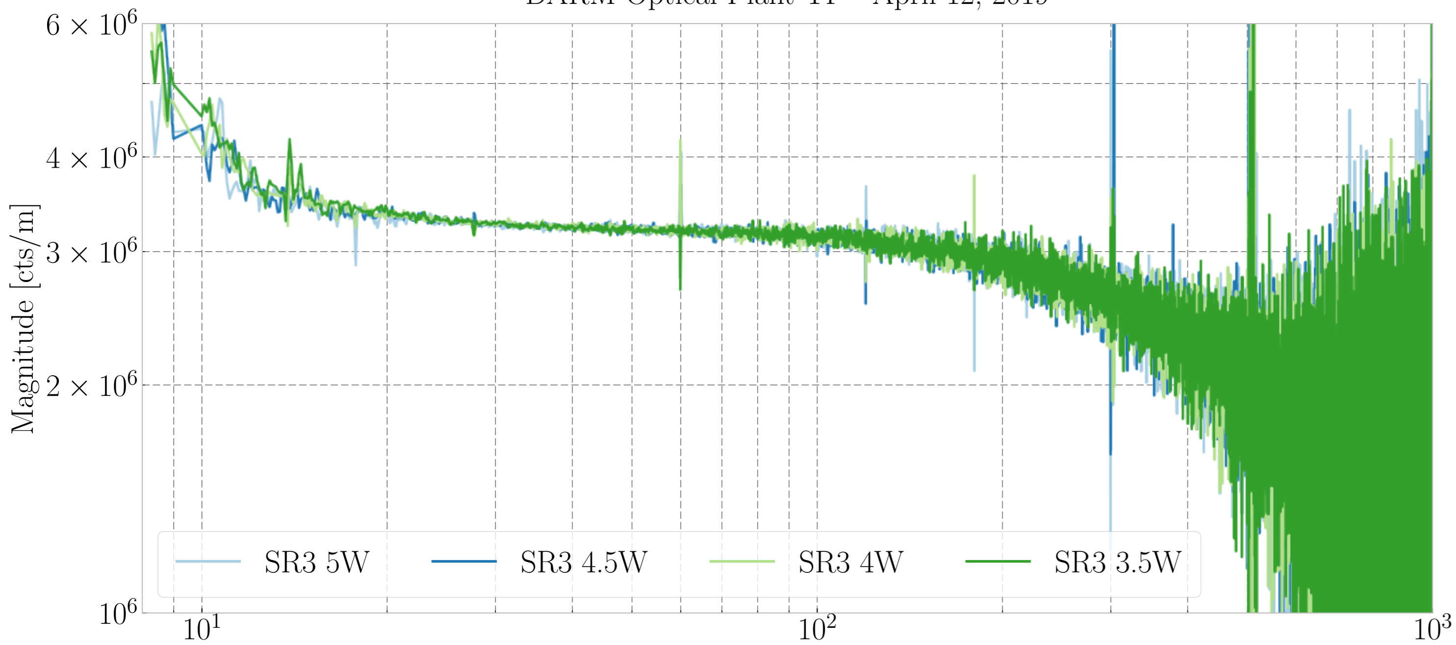
DARM Optical Plant TF - April 12, 2019
