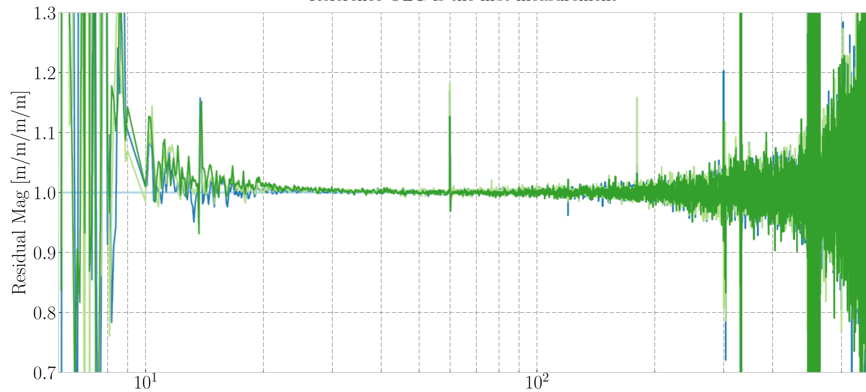
DARM OLG Residuals - March 15, 2019 Reference OLG is the first measurement
