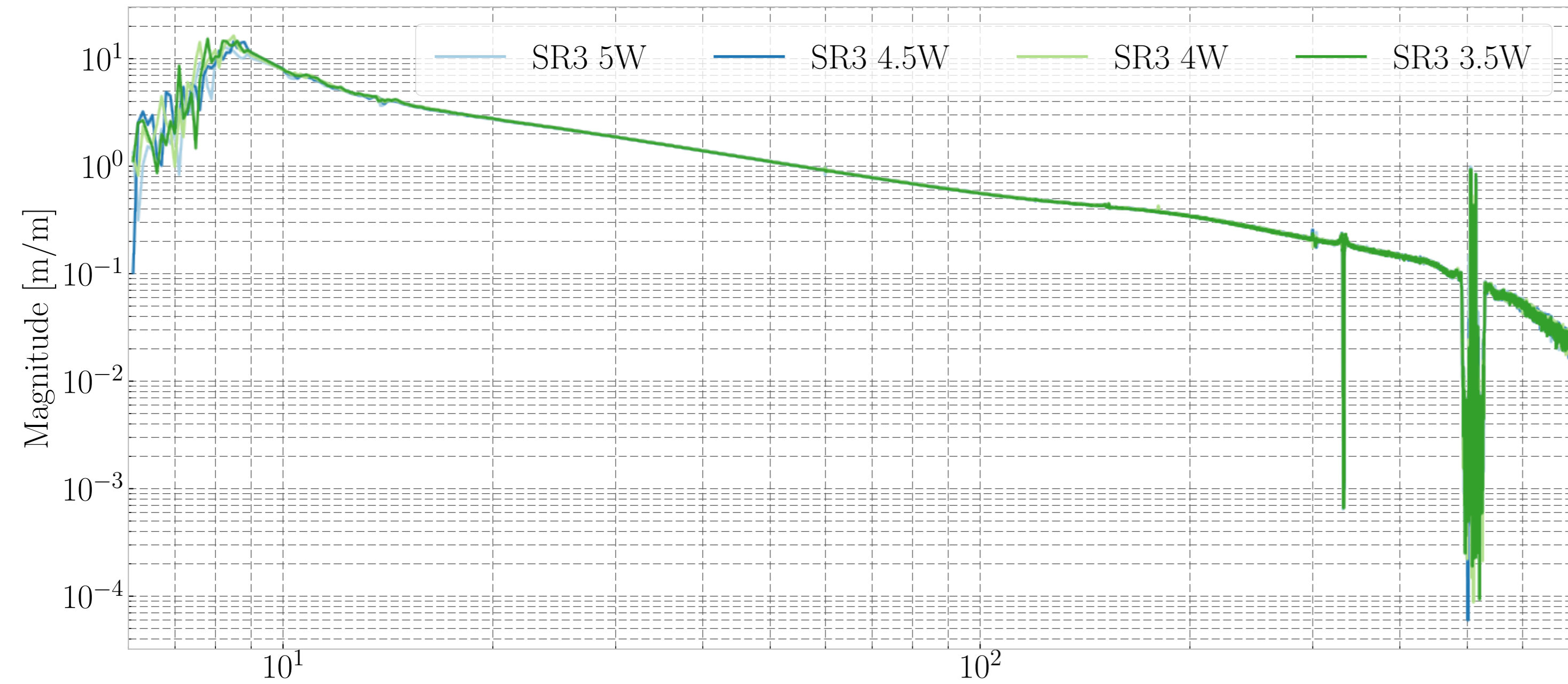
DARM OLG - April 12, 2019
