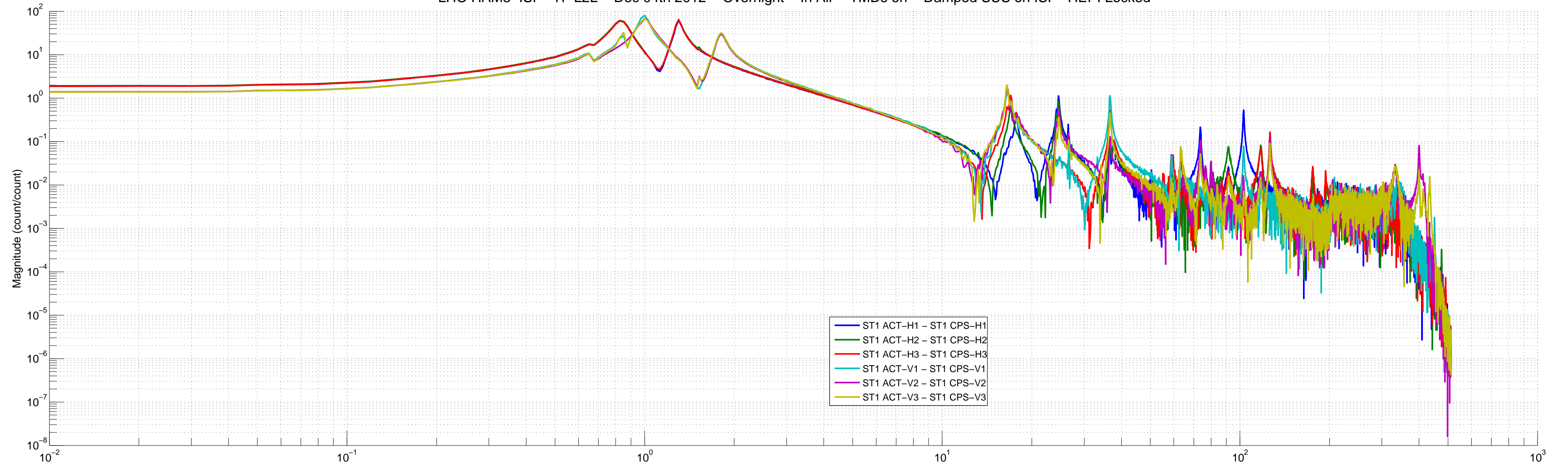
LHO HAM3-ISI - TF L2L - Dec 04th 2012 - Overnight - In Air - TMDs on - Damped SUS on ISI - HEPI Locked
