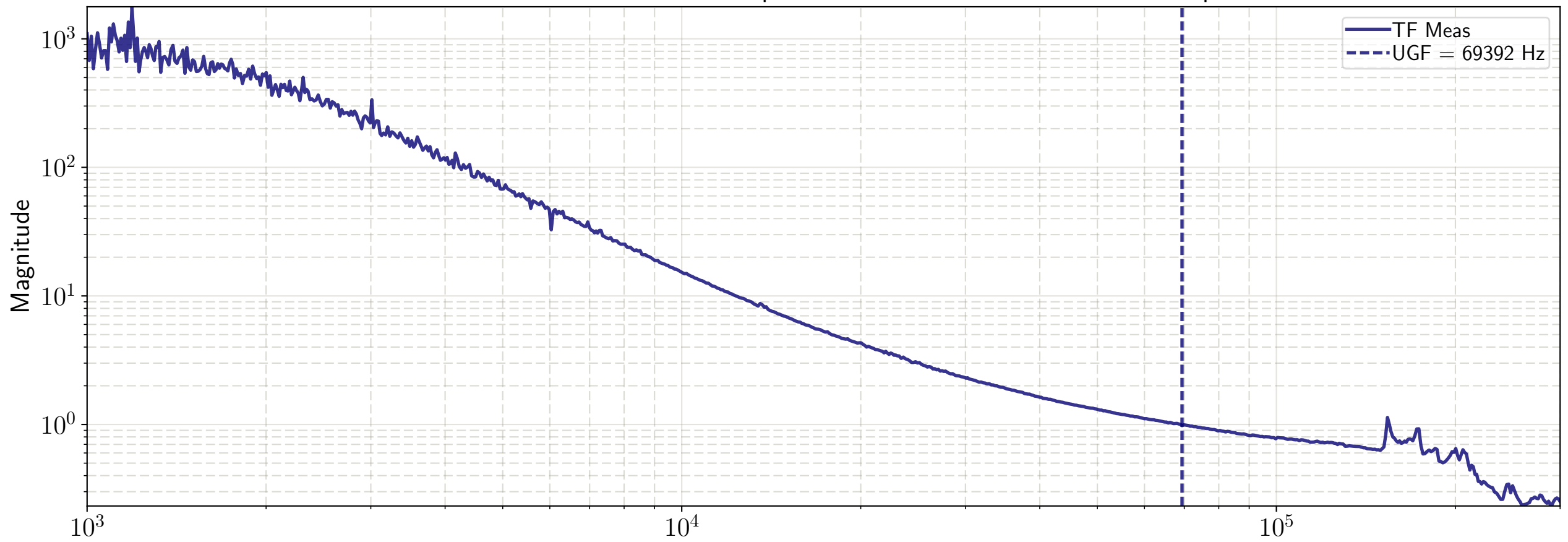
IMC OLG - IMC Locked Alone - 35W Input - IN1 +22dB - Second Boost On - Apr-23-2019
