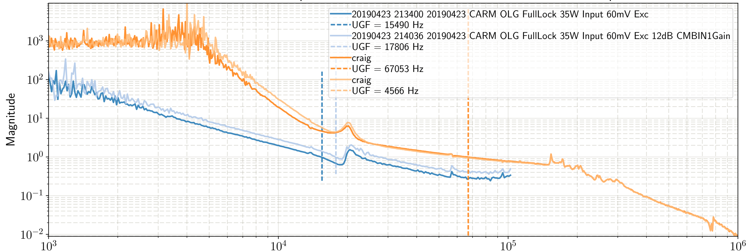
CARM + IMC OLGs Full Lock - Input 35 W - CMB IN1 slider moved from +9dB to +12dB - Apr-23-2019
