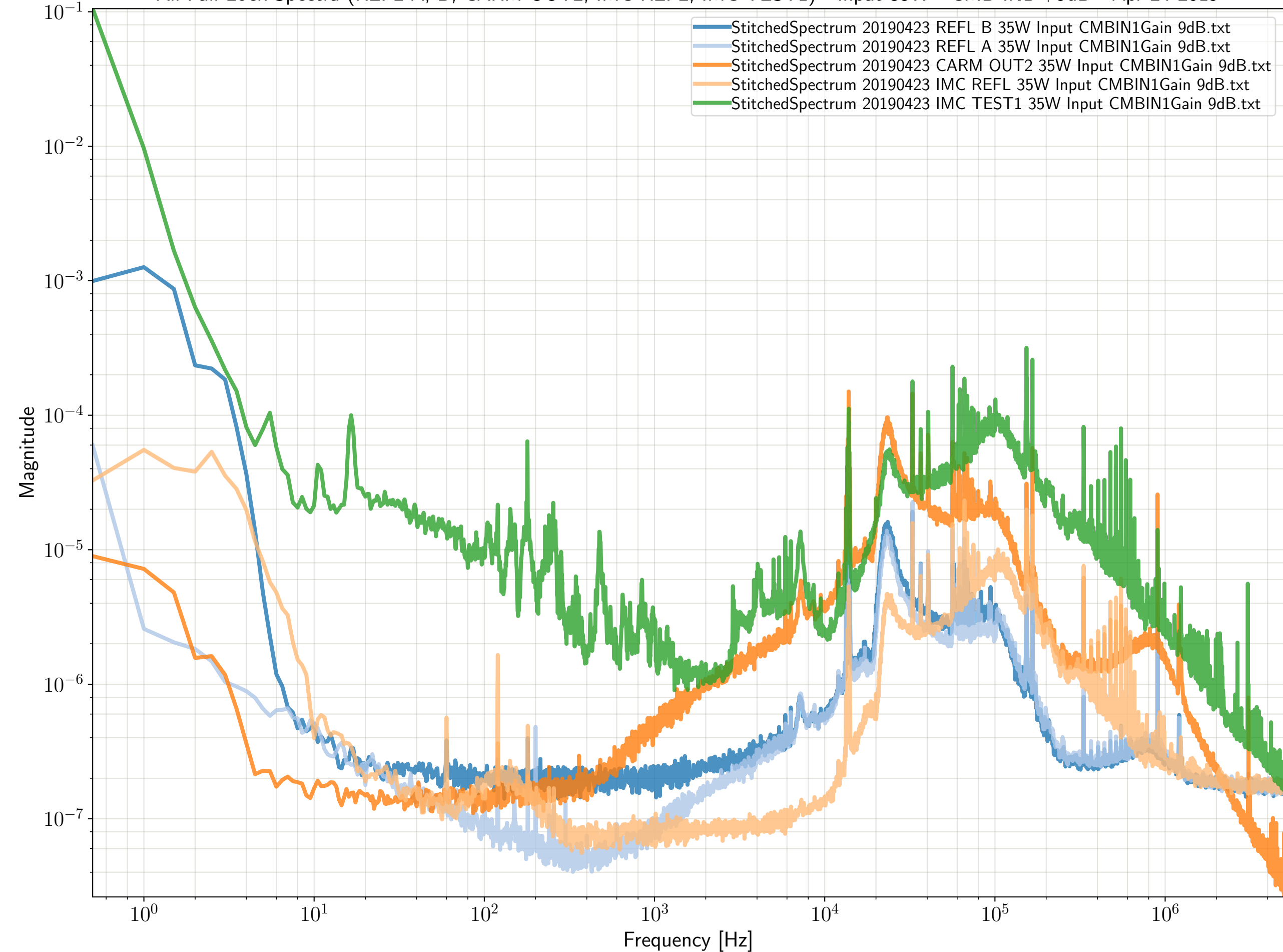
All Full Lock Spectra (REFL A, B, CARM OUT2, IMC REFL, IMC TEST1) - Input 35W - CMB IN1 +9dB - Apr-24-2019
